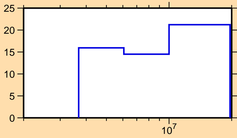
\Delta\sigma/\sigma vs. E for ^{146}\text{La}(n,el.)
