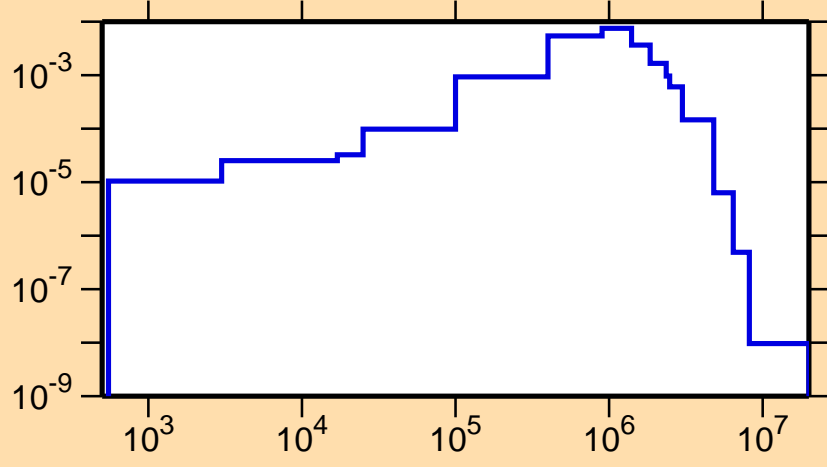
\sigma vs. E for ^{146}\text{La}(n,n_2)
