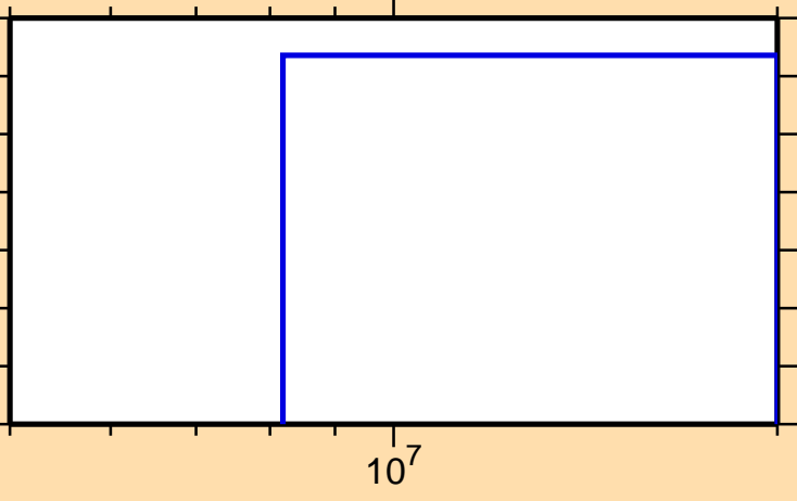
\sigma vs. E for ^{146}\text{La}(n,3n\alpha)
