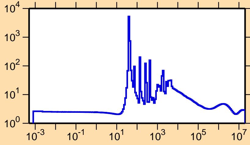
\sigma vs. E for ^{147}\text{La}(n,\text{el.})
