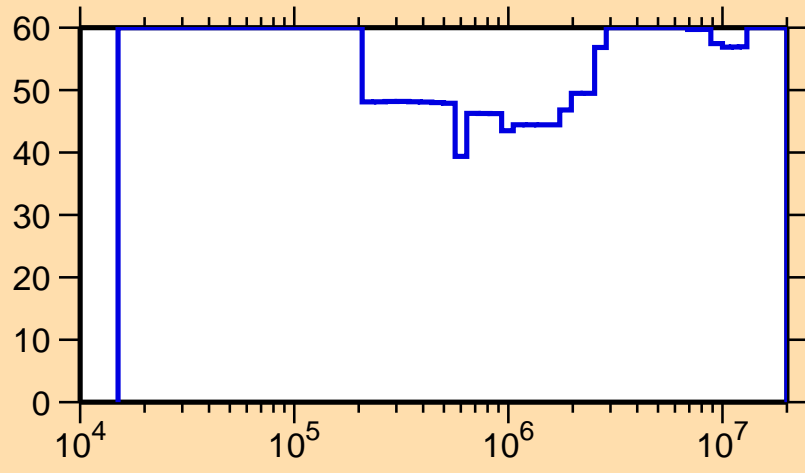
\Delta\sigma/\sigma vs. E for ^{147}\text{La}(n,n_1)
