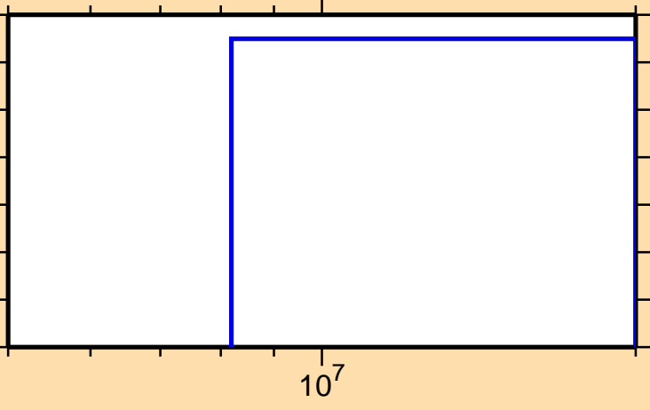
\sigma vs. E for ^{147}\text{La}(n,2np)
