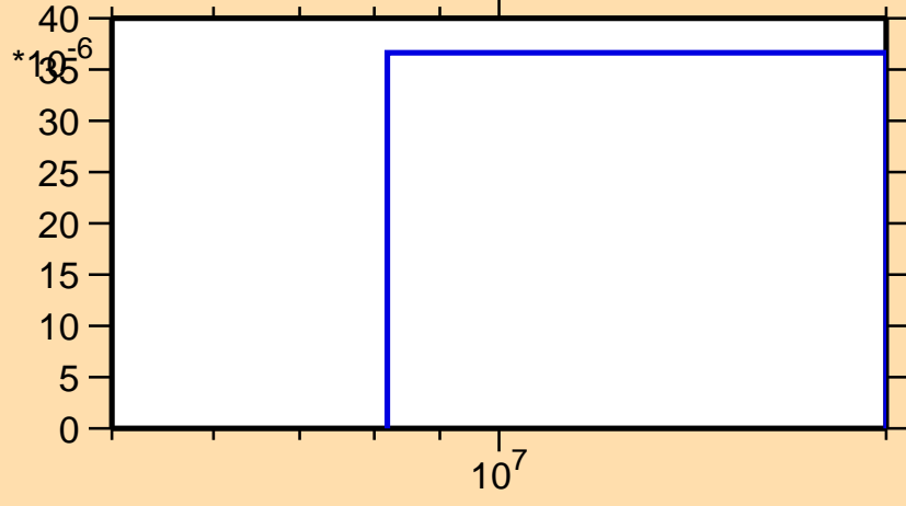
\sigma vs. E for ^{147}\text{La}(n,t)
