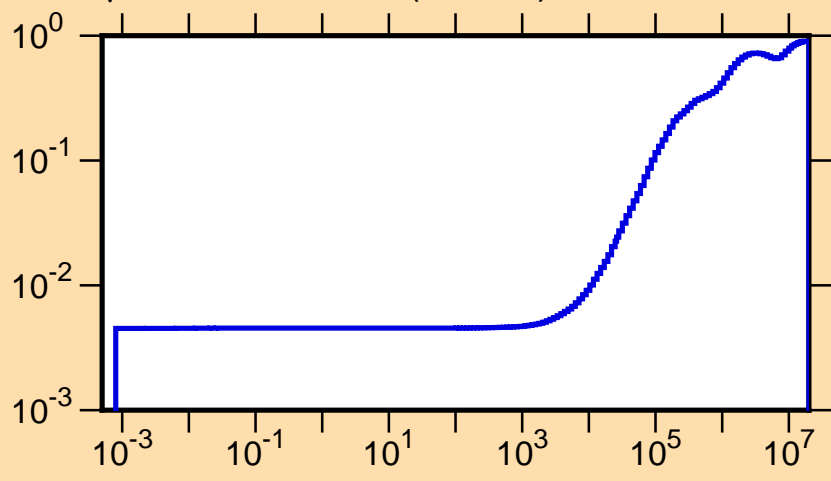
\mu vs. E for ^{149}\text{La}(\text{mt251})
