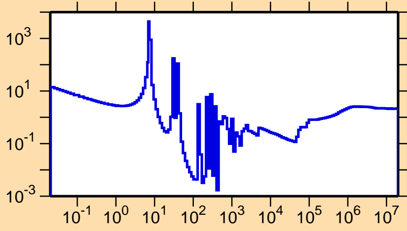
\sigma vs. E for ^{149}\text{La}(n,\text{nonel.})
