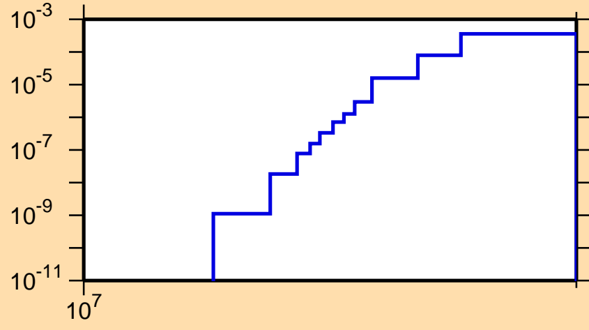
\sigma vs. E for ^{149}\text{La}(n,np)
