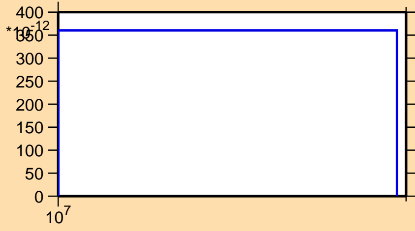
\sigma vs. E for ^{149}\text{La}(n,2n\alpha)
