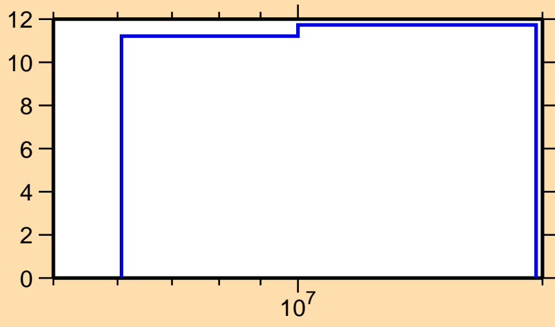
\Delta\sigma/\sigma vs. E for ^{149}\text{La}(n,el.)
