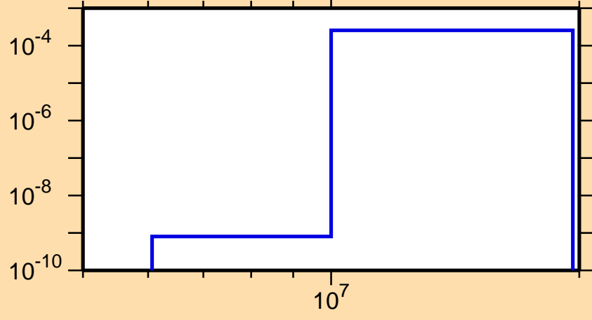
\sigma vs. E for ^{149}\text{La}(n,p)
