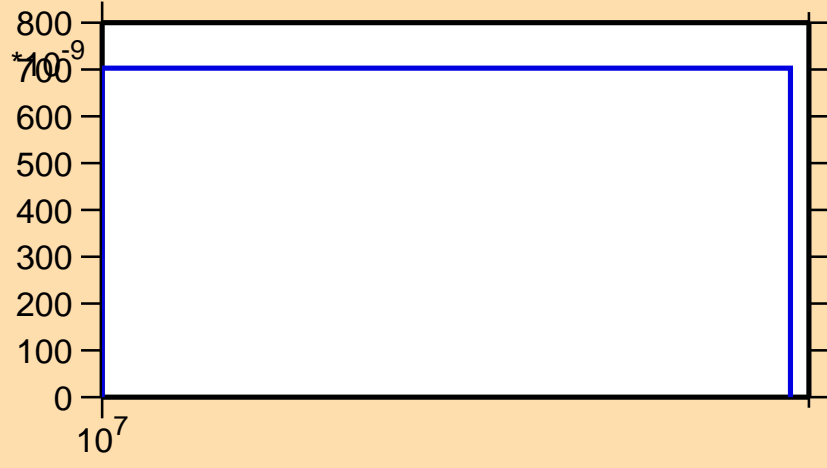
\sigma vs. E for ^{149}\text{La}(n,nt)
