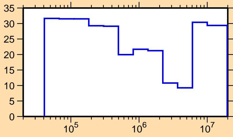
\Delta\sigma/\sigma vs. E for ^{149}\text{La}(n,\text{inel.})
