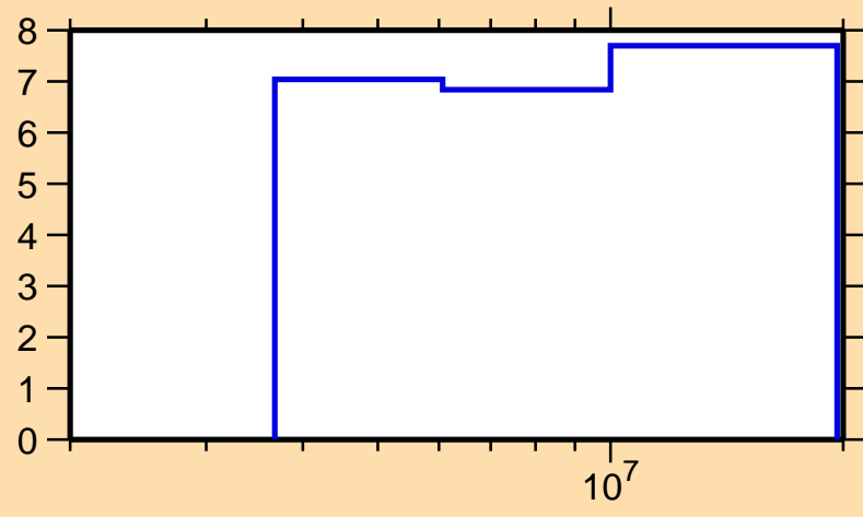
\Delta\sigma/\sigma vs. E for ^{149}\text{La}(n,\text{nonel.})
