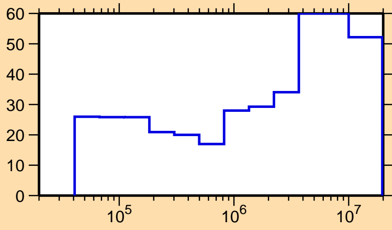
\Delta\sigma/\sigma vs. E for ^{149}\text{La}(n,n_1)
