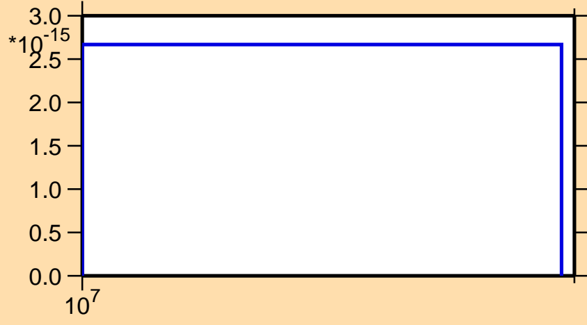
\sigma vs. E for ^{149}\text{La}(n,3n\alpha)
