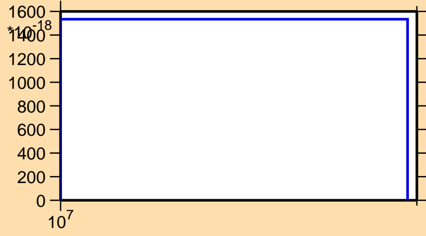
\sigma vs. E for ^{149}\text{La} (mt 11)
