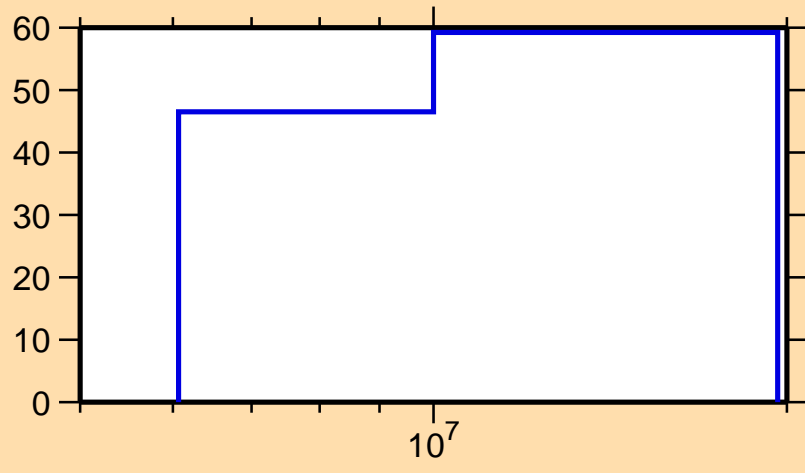
\Delta\sigma/\sigma vs. E for ^{149}\text{La}(n,n\text{cont.})
