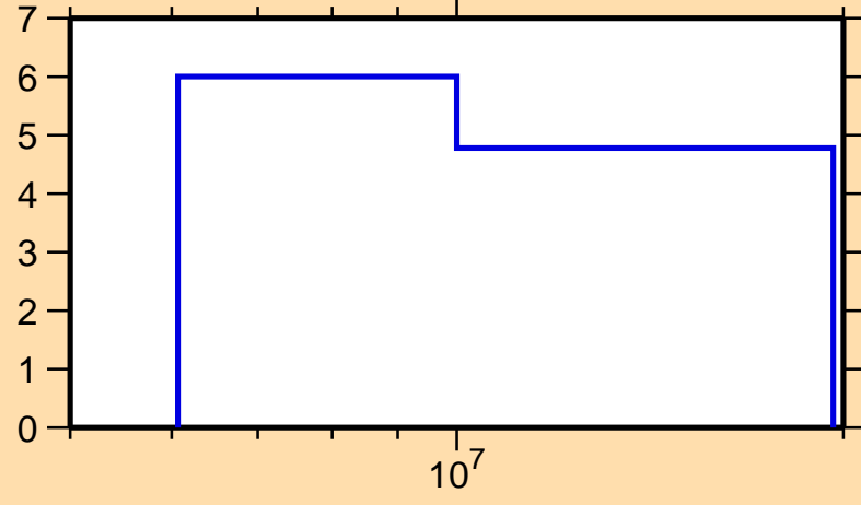
\Delta\sigma/\sigma vs. E for ^{149}\text{La}(n,\text{tot.})
