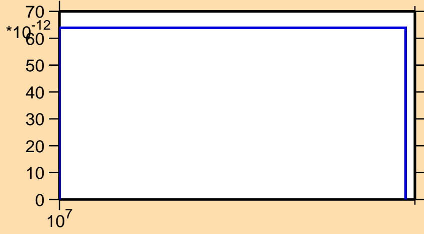
\sigma vs. E for ^{149}\text{La}(n,2np)
