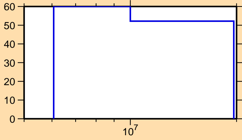
\Delta\sigma/\sigma vs. E for ^{149}\text{La}(n,n_1)
