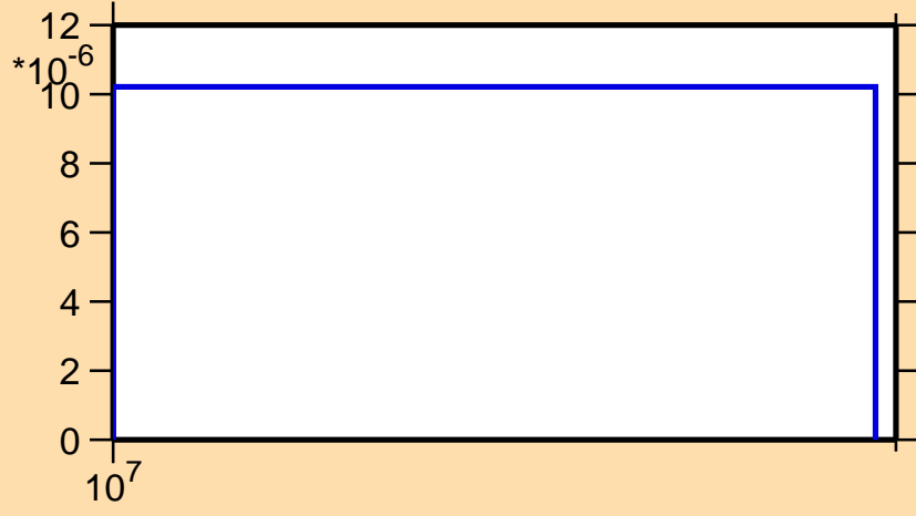
\sigma vs. E for ^{149}\text{La}(n,np)
