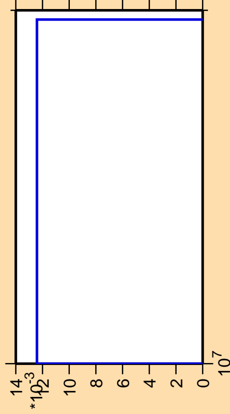
\Delta\sigma/\sigma vs. E for ^{149}\text{La} (mt 11)
