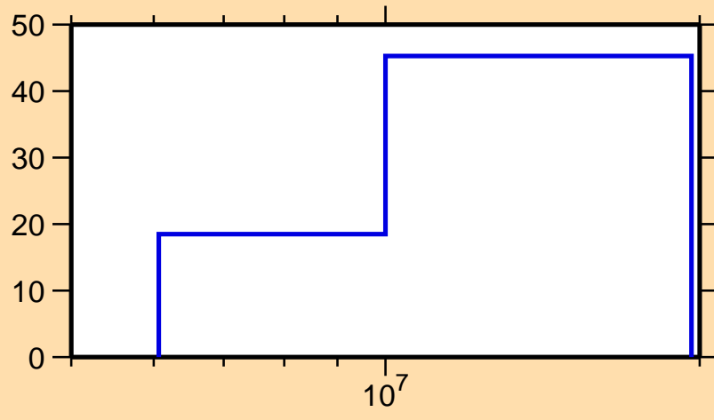
\Delta\sigma/\sigma vs. E for ^{149}\text{La}(n,2n)
