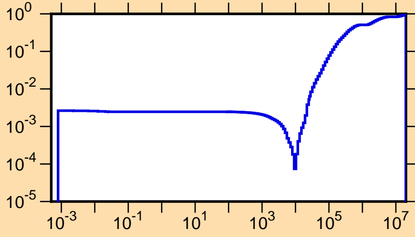
\mu vs. E for ^{254}\text{Lw}(\text{mt251})
