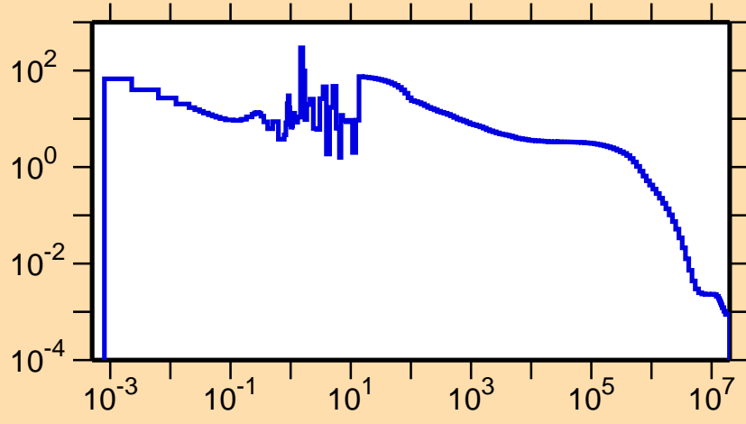
\sigma vs. E for ^{254}\text{Lw}(n,\gamma)
