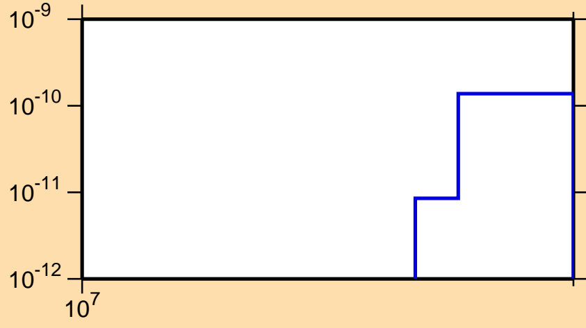
\sigma vs. E for ^{254}\text{Lw} (mt 34)
