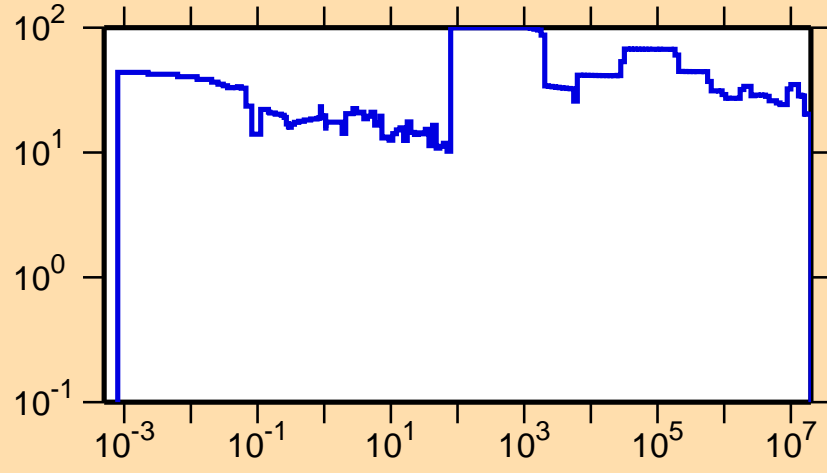
\Delta\sigma/\sigma vs. E for ^{255}\text{Lw}(n,tot.)
