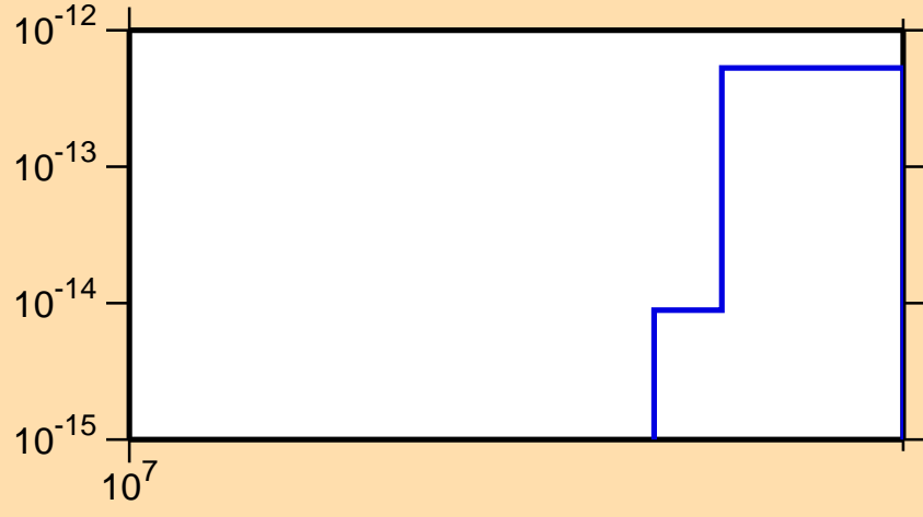
\sigma vs. E for ^{255}\text{Lw}(n,\text{pt})
