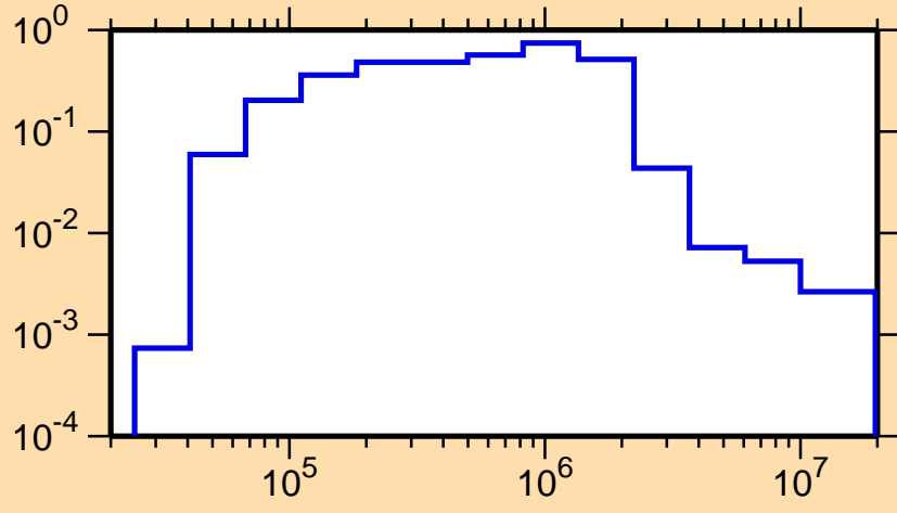
\sigma vs. E for ^{255}\text{Lw}(n,n_1)
