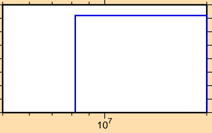
\sigma vs. E for ^{255}\text{Lw}(n,\text{pd})
