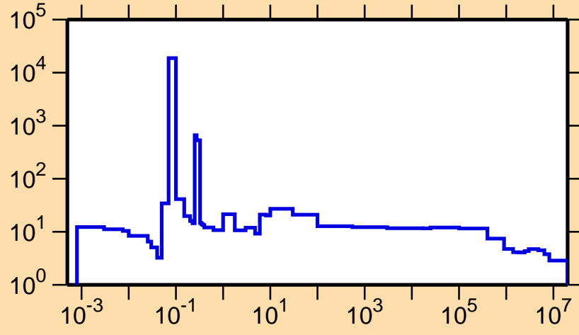
\sigma vs. E for ^{255}\text{Lw}(n,\text{el.})
