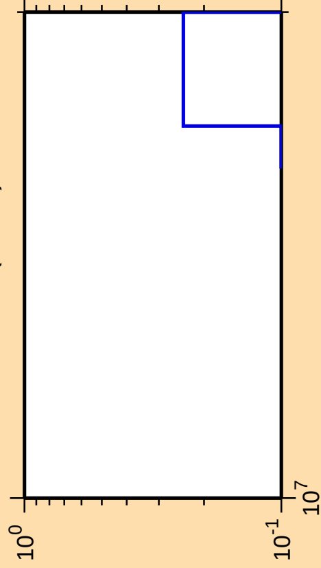
\Delta\sigma/\sigma vs. E for ^{255}\text{Lw}(\text{mt 11})
