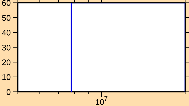
\Delta\sigma/\sigma vs. E for ^{255}\text{Lw}(n,2n)
