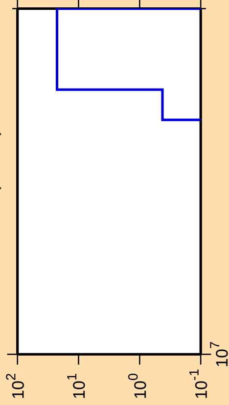
\Delta\sigma/\sigma vs. E for ^{255}\text{Lw}(\text{mt 34})
