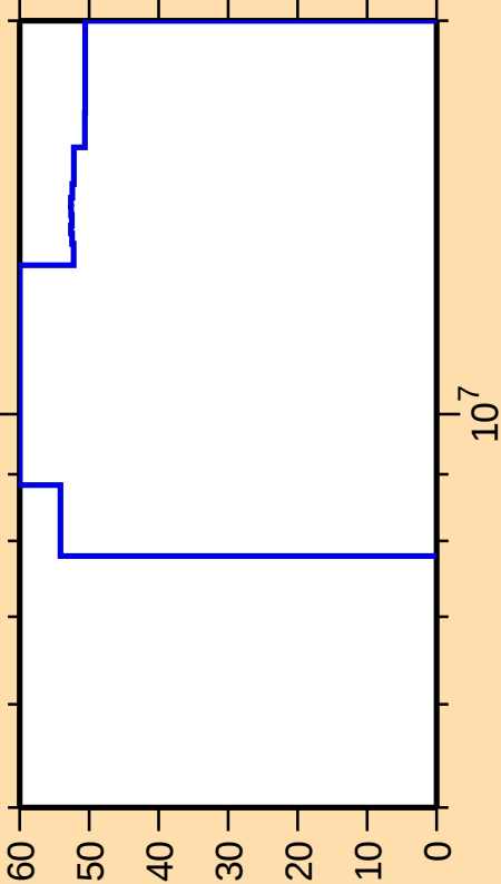
\Delta\sigma/\sigma vs. E for ^{255}\text{Lw}(n,n\text{cont.})
