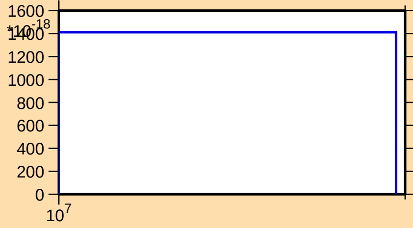
\sigma vs. E for ^{255}\text{Lw}(\text{mt 11})
