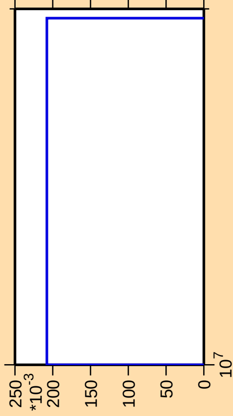
\Delta\sigma/\sigma vs. E for ^{255}\text{Lw}(\text{mt } 34)
