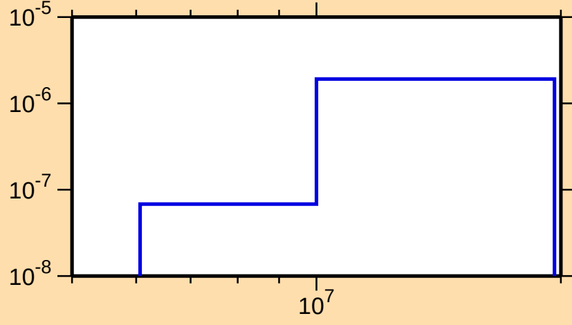
\sigma vs. E for ^{255}\text{Lw}(n,2n\alpha)
