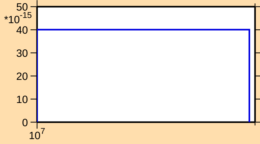
\sigma vs. E for ^{255}\text{Lw}(\text{mt } 34)
