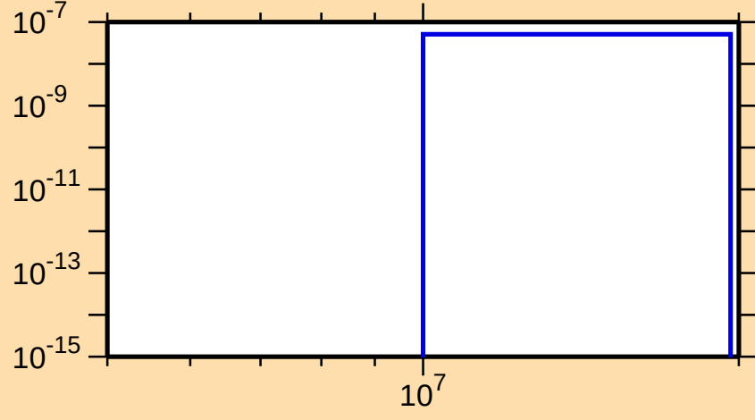
\sigma vs. E for ^{255}\text{Lw}(\text{mt117})
