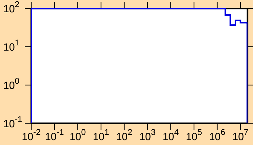
\Delta\sigma/\sigma vs. E for ^{255}\text{Lw}(n,p)
