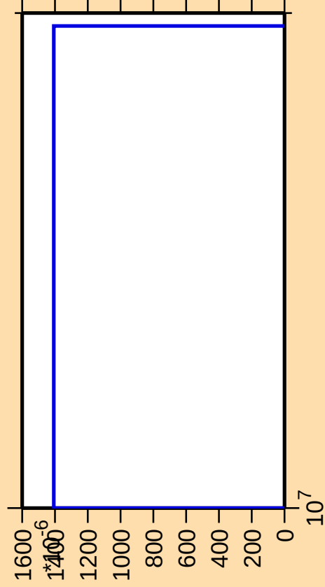
\Delta\sigma/\sigma vs. E for ^{255}\text{Lw}(\text{mt 11})
