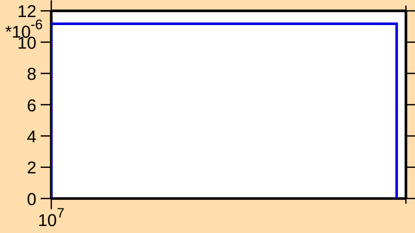
\sigma vs. E for ^{255}\text{Lw}(n,3n\alpha)
