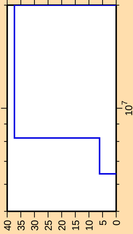
\Delta\sigma/\sigma vs. E for ^{255}\text{Lw}(n,t)
