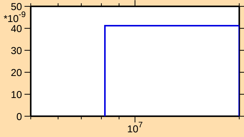
\sigma vs. E for ^{255}\text{Lw}(\text{mt117})
