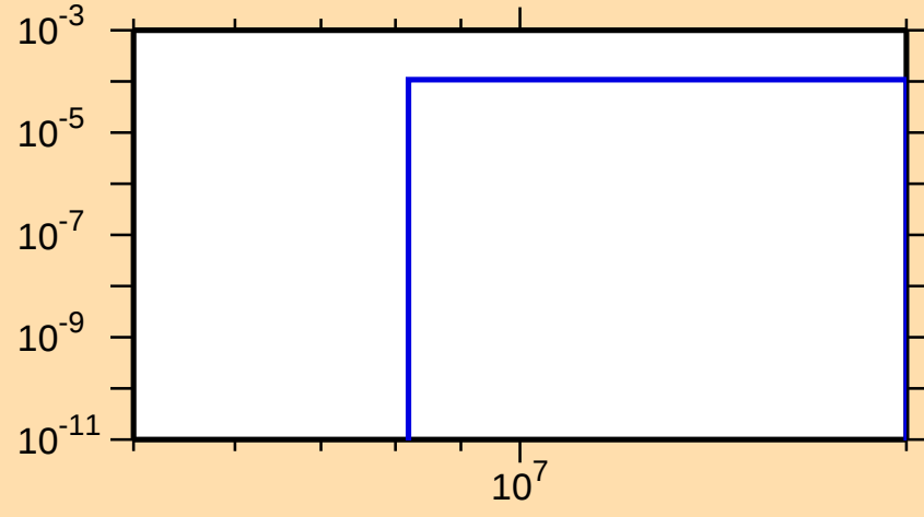
\sigma vs. E for ^{255}\text{Lw}(n,t)
