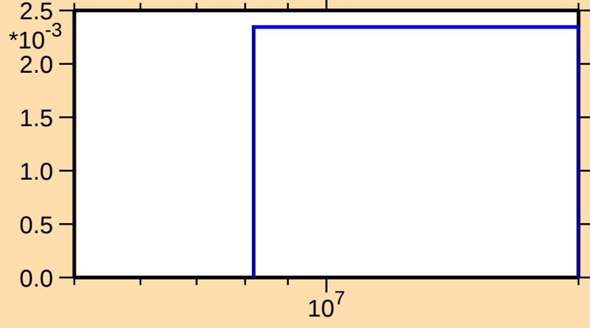
\sigma vs. E for ^{255}\text{Lw}(n,3n)
