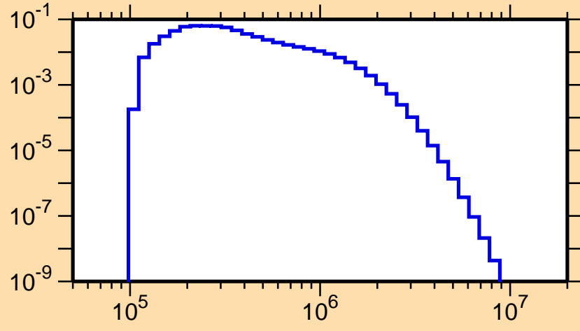
\sigma vs. E for ^{256}\text{Lw}(n, n_1)
