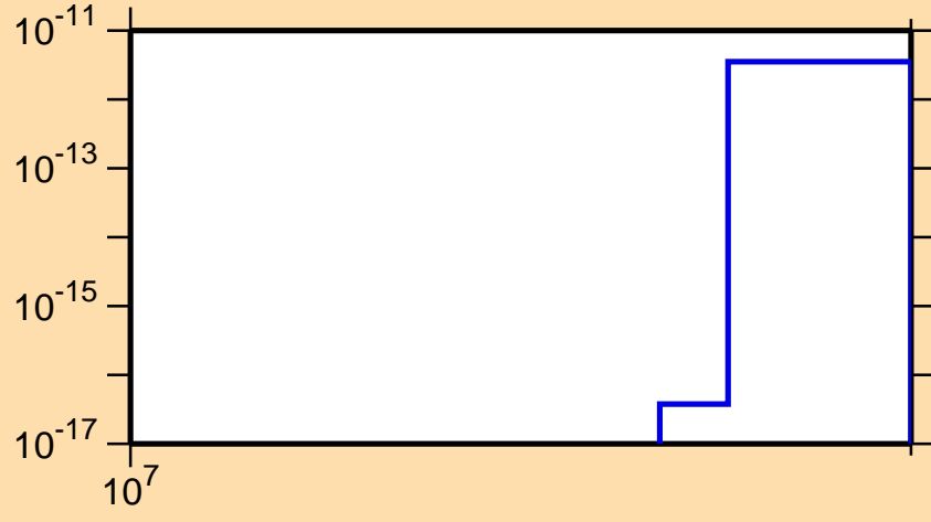
\sigma vs. E for ^{256}\text{Lw} (mt 11)
