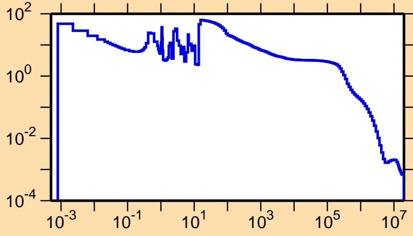
\sigma vs. E for ^{256}\text{Lw}(n,\gamma)
