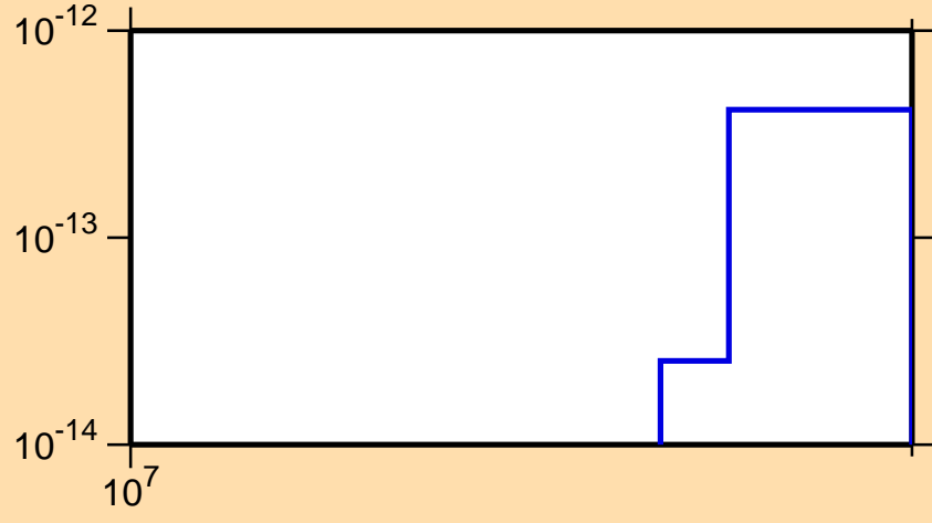
\sigma vs. E for ^{256}\text{Lw}(n,pt)
