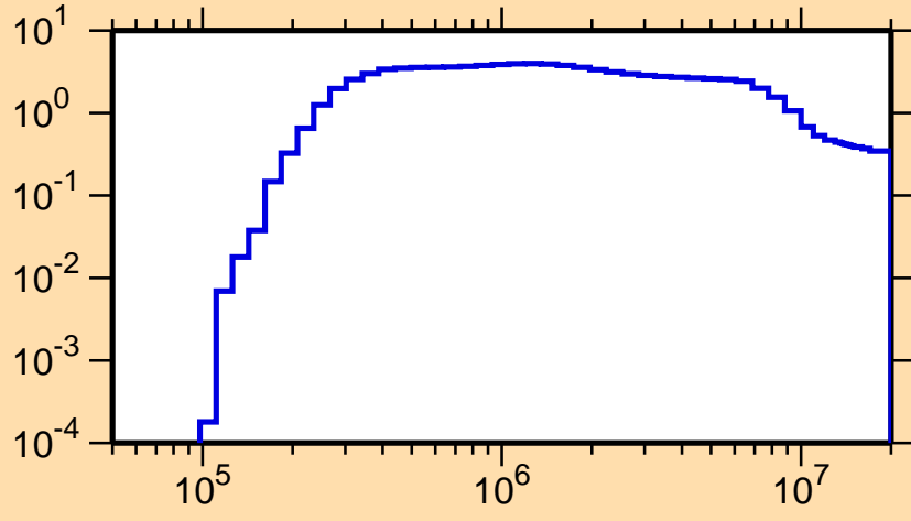
\sigma vs. E for ^{256}\text{Lw}(n,\text{inel.})
