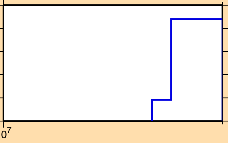
\sigma vs. E for ^{256}\text{Lw} (mt 42)
