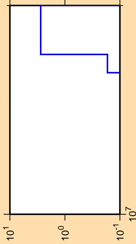
\Delta\sigma/\sigma vs. E for ^{256}\text{Lw}(n,pt)
