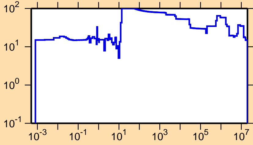
\Delta\sigma/\sigma vs. E for ^{256}\text{Lw}(n,el.)
