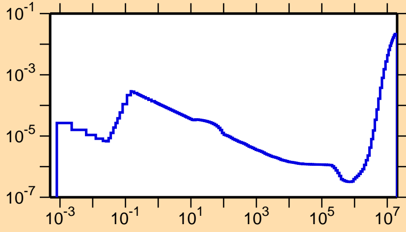
\sigma vs. E for ^{256}\text{Lw}(n,p)
