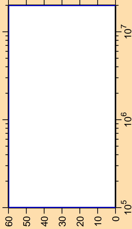
\Delta\sigma/\sigma vs. E for ^{256}\text{Lw}(n,\alpha)
