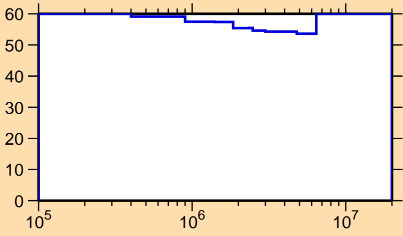
\Delta\sigma/\sigma vs. E for ^{256}\text{Lw}(n,n\text{cont.})
