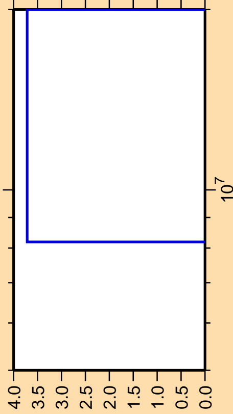
\Delta\sigma/\sigma vs. E for ^{256}\text{Lw}(\text{mt 34})
