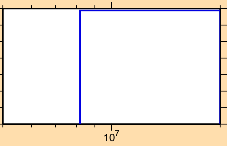
\sigma vs. E for ^{256}\text{Lw}(n,3n\alpha)
