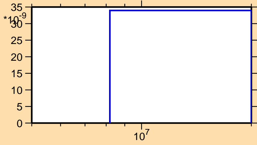
\sigma vs. E for ^{256}\text{Lw}(\text{mt117})
