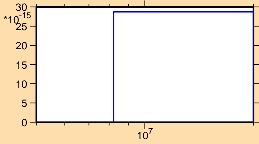
\sigma vs. E for ^{256}\text{Lw}(\text{mt } 11)
