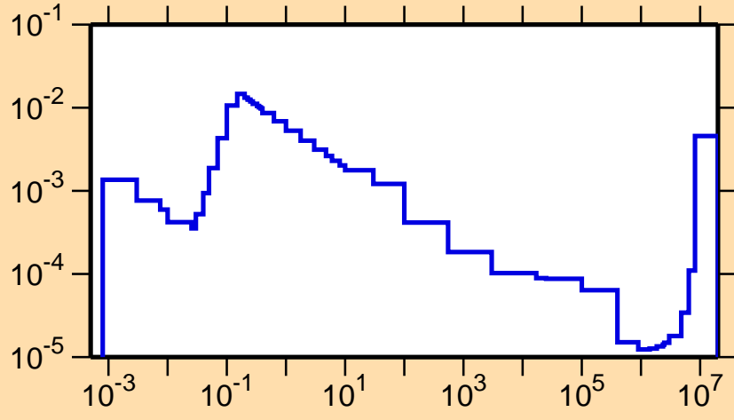
\sigma vs. E for ^{256}\text{Lw}(n,\alpha)
