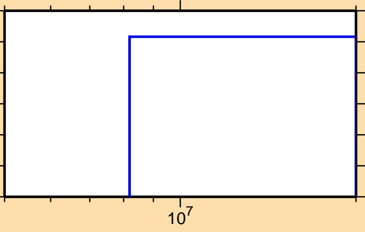
\sigma vs. E for ^{256}\text{Lw}(\text{mt 34})
