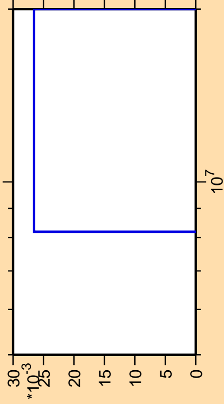
\Delta\sigma/\sigma vs. E for ^{256}\text{Lw}(\text{mt } 11)
