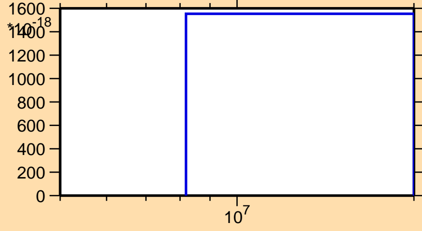
\sigma vs. E for ^{256}\text{Lw}(n,\text{pd})
