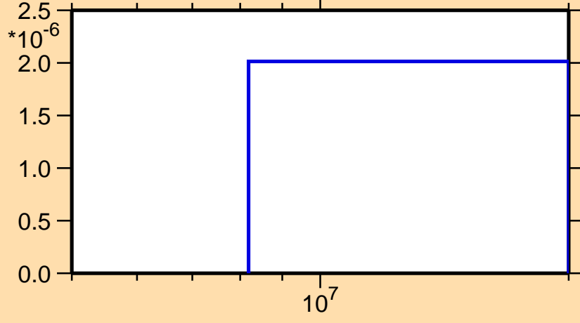
\sigma vs. E for ^{256}\text{Lw}(n,2np)
