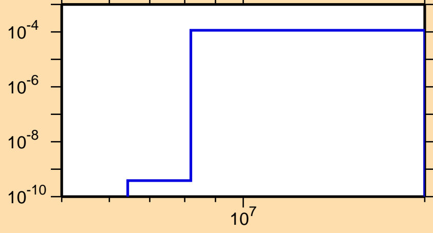
\sigma vs. E for ^{256}\text{Lw}(n,2n\alpha)
