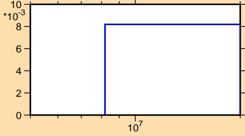
\sigma vs. E for ^{256}\text{Lw}(n,3n)
