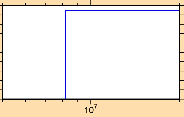
\sigma vs. E for ^{256}\text{Lw}(n,nd)
