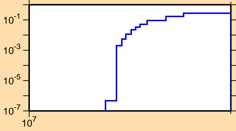
\sigma vs. E for ^{257}\text{Lw}(n,3n)
