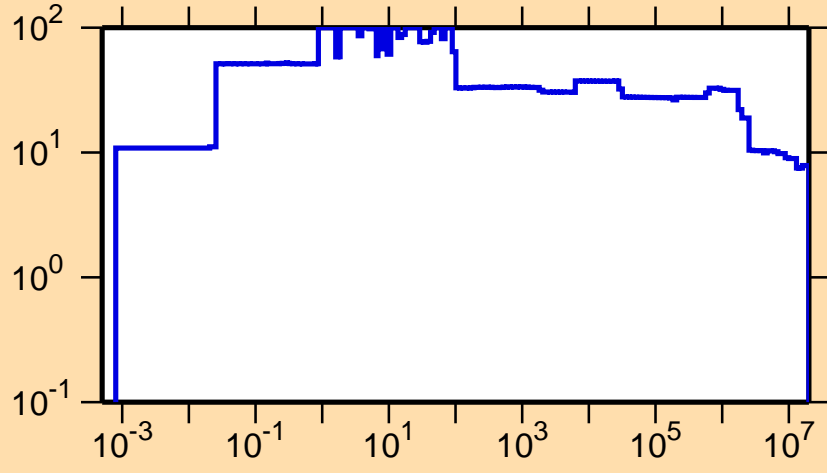
\Delta\sigma/\sigma vs. E for ^{257}\text{Lw}(n,\text{nonel.})
