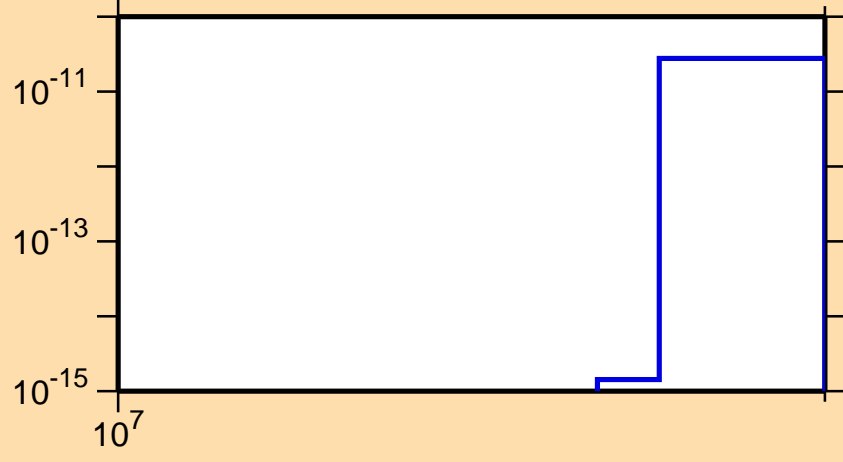
\sigma vs. E for ^{257}\text{Lw} (mt 11)
