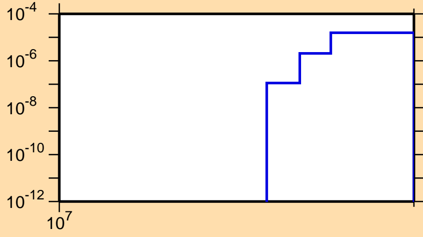
\sigma vs. E for ^{257}\text{Lw}(n,3n\alpha)
