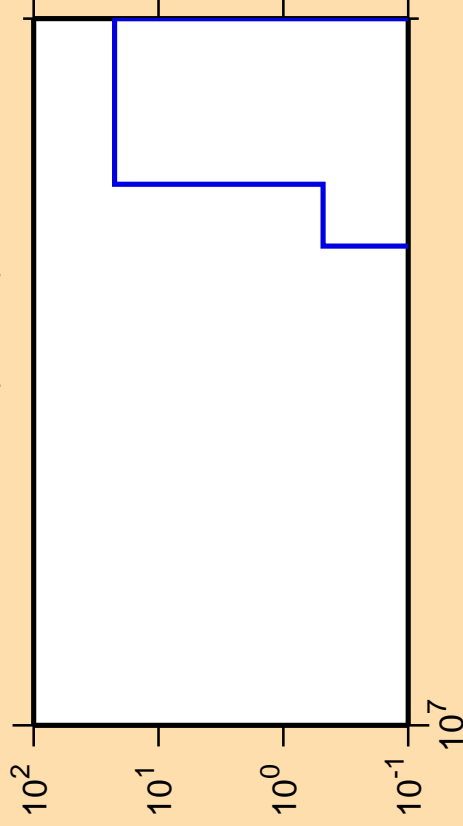
\Delta\sigma/\sigma vs. E for ^{257}\text{Lw} (mt 34)
