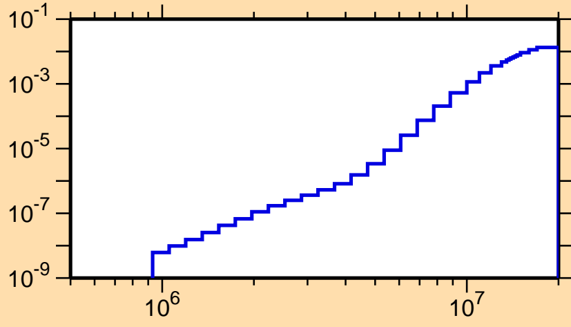
\sigma vs. E for ^{257}\text{Lw}(n,p)
