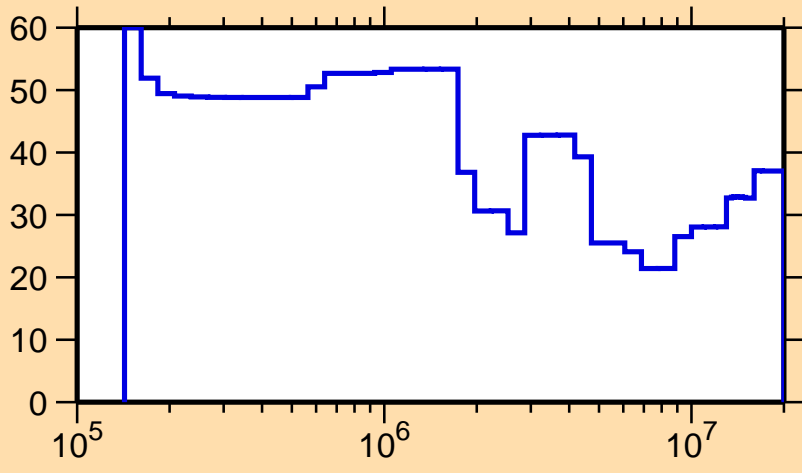
\Delta\sigma/\sigma vs. E for ^{257}\text{Lw}(n,n_1)
