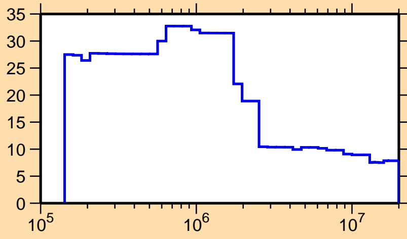
\Delta\sigma/\sigma vs. E for ^{257}\text{Lw}(n,\text{nonel.})
