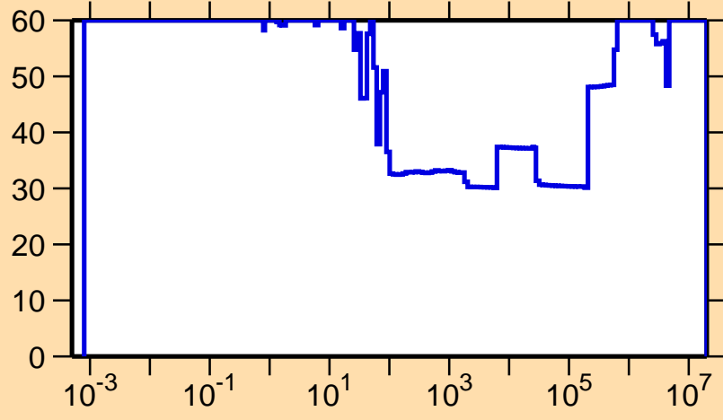
\Delta\sigma/\sigma vs. E for ^{257}\text{Lw}(n,\gamma)
