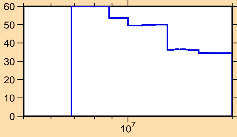
\Delta\sigma/\sigma vs. E for ^{257}\text{Lw}(n,\text{inel.})
