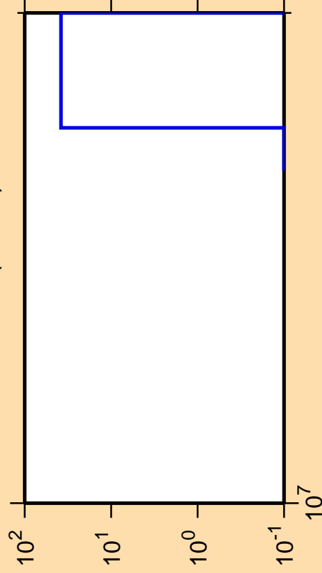
\Delta\sigma/\sigma vs. E for ^{257}\text{Lw} (mt 11)
