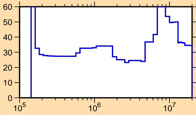
\Delta\sigma/\sigma vs. E for ^{257}\text{Lw}(n,\text{inel.})
