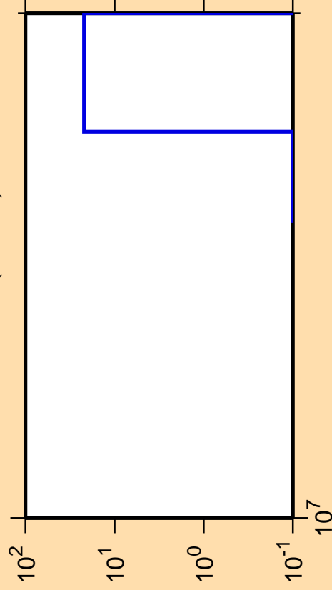
\Delta\sigma/\sigma vs. E for ^{257}\text{Lw} (mt 42)
