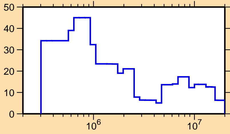
\Delta\sigma/\sigma vs. E for ^{257}\text{Lw}(n,\text{el.})
