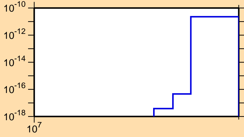
\sigma vs. E for ^{257}\text{Lw} (mt 42)
