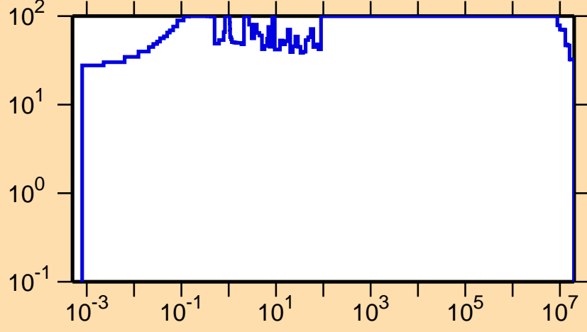
\Delta\sigma/\sigma vs. E for ^{257}\text{Lw}(n,f)
