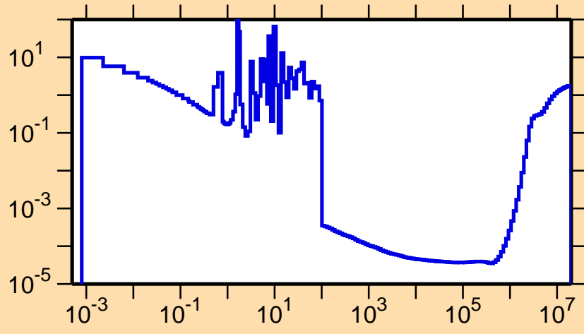
\sigma vs. E for ^{257}\text{Lw}(n,f)
