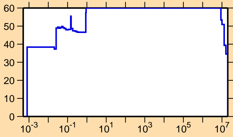
\Delta\sigma/\sigma vs. E for ^{257}\text{Lw}(n,p)
