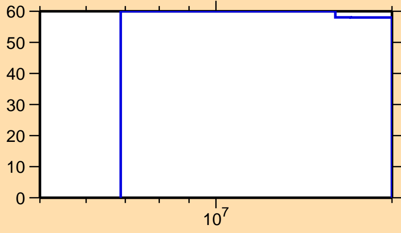
\Delta\sigma/\sigma vs. E for ^{257}\text{Lw}(n,2n)
