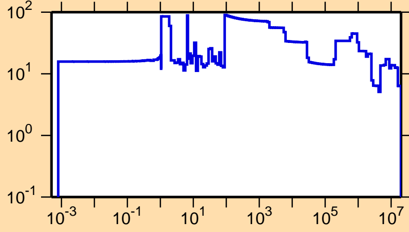
\Delta\sigma/\sigma vs. E for ^{257}\text{Lw}(n,\text{el.})
