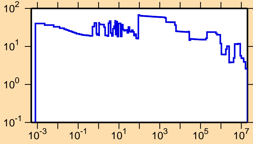
\Delta\sigma/\sigma vs. E for ^{257}\text{Lw}(n,\text{tot.})
