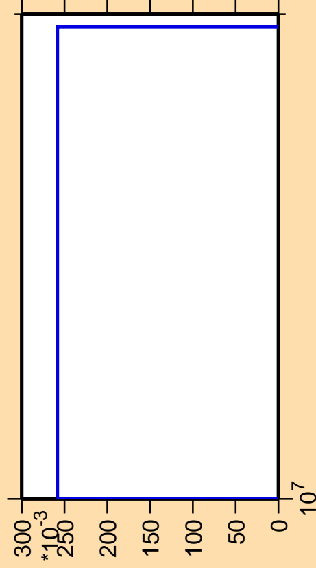
\Delta\sigma/\sigma vs. E for ^{257}\text{Lw} (mt 11)
