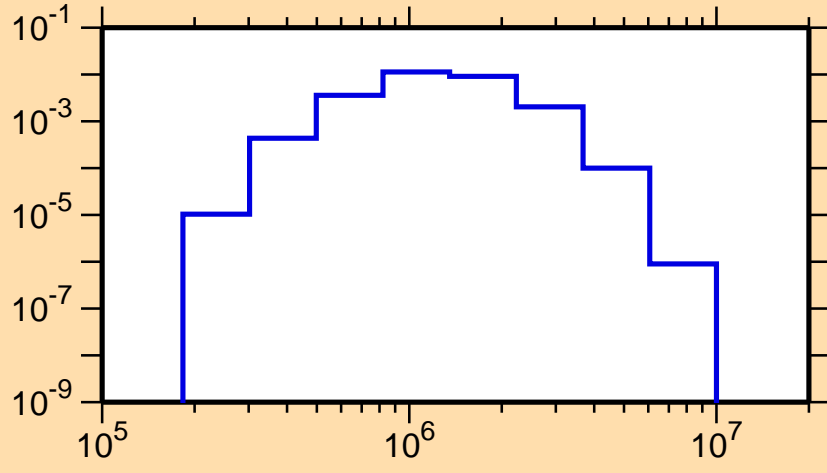
\sigma vs. E for ^{257}\text{Lw}(n, n_2)
