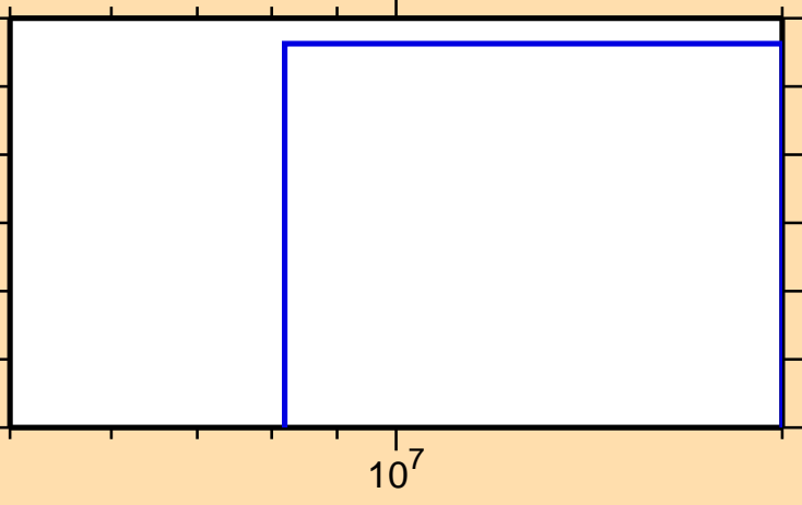
\sigma vs. E for ^{257}\text{Lw}(\text{mt117})
