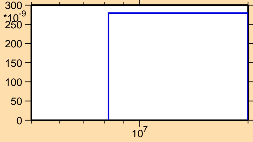
\sigma vs. E for ^{257}\text{Lw}(n,nt)
