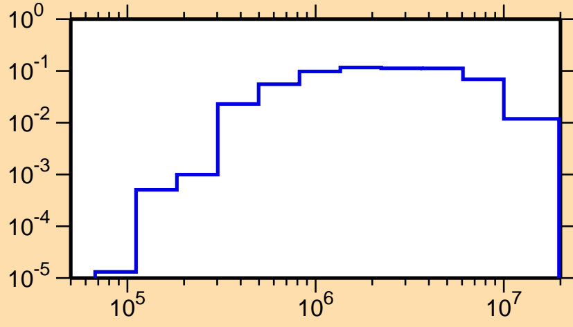
\sigma vs. E for ^{258}\text{Lw}(n,n\alpha)
