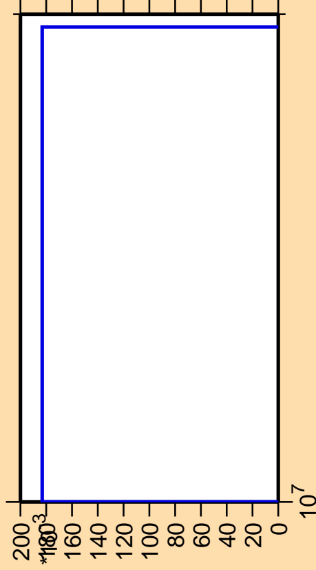
\Delta\sigma/\sigma vs. E for ^{258}\text{Lw}(\text{mt 11})
