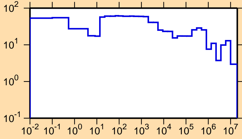
\Delta\sigma/\sigma vs. E for ^{258}\text{Lw}(n,\text{tot.})
