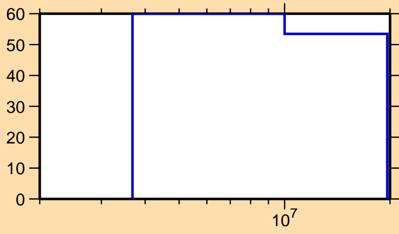
\Delta\sigma/\sigma vs. E for ^{258}\text{Lw}(n,2n)
