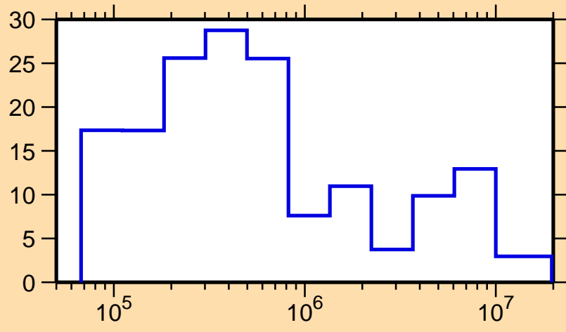
\Delta\sigma/\sigma vs. E for ^{258}\text{Lw}(n,\text{tot.})
