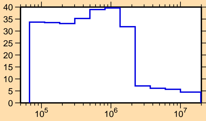
\Delta\sigma/\sigma vs. E for ^{258}\text{Lw}(n,\text{nonel.})
