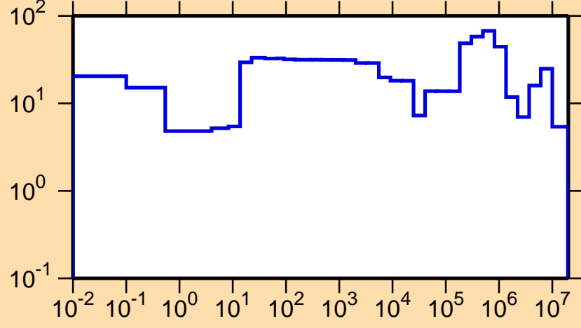
\Delta\sigma/\sigma vs. E for ^{258}\text{Lw}(n,\text{el.})
