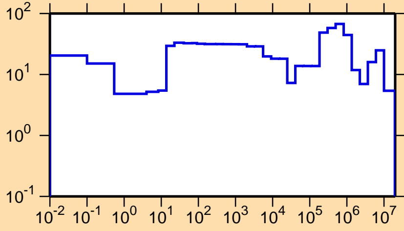
\Delta\sigma/\sigma vs. E for ^{258}\text{Lw}(n,el.)
