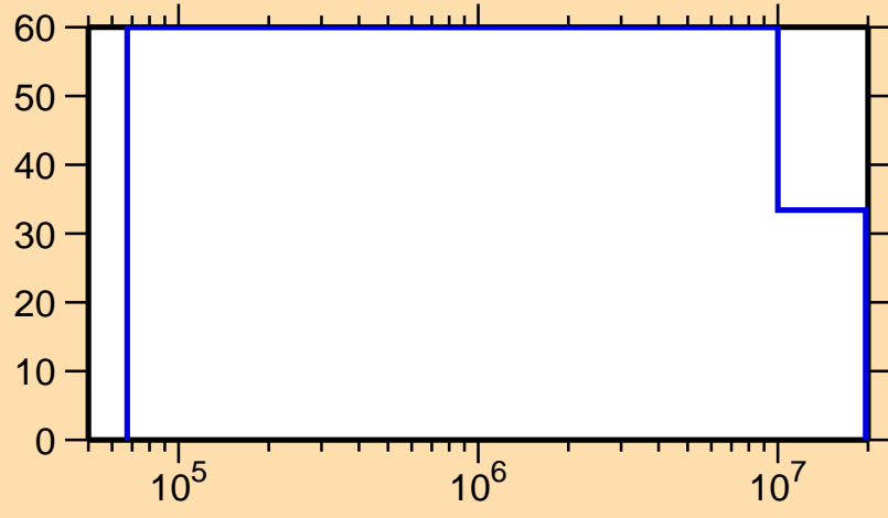
\Delta\sigma/\sigma vs. E for ^{258}\text{Lw}(n,f)
