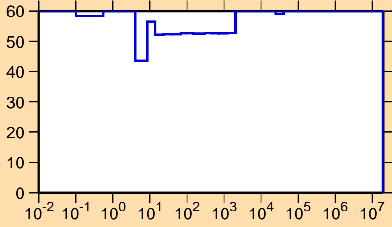
\Delta\sigma/\sigma vs. E for ^{258}\text{Lw}(n,\gamma)
