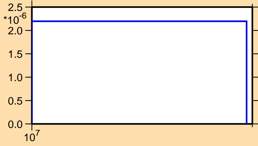
\sigma vs. E for ^{258}\text{Lw}(n,3n\alpha)
