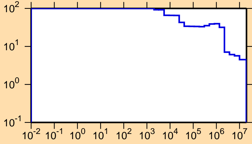
\Delta\sigma/\sigma vs. E for ^{258}\text{Lw}(n,\text{nonel.})
