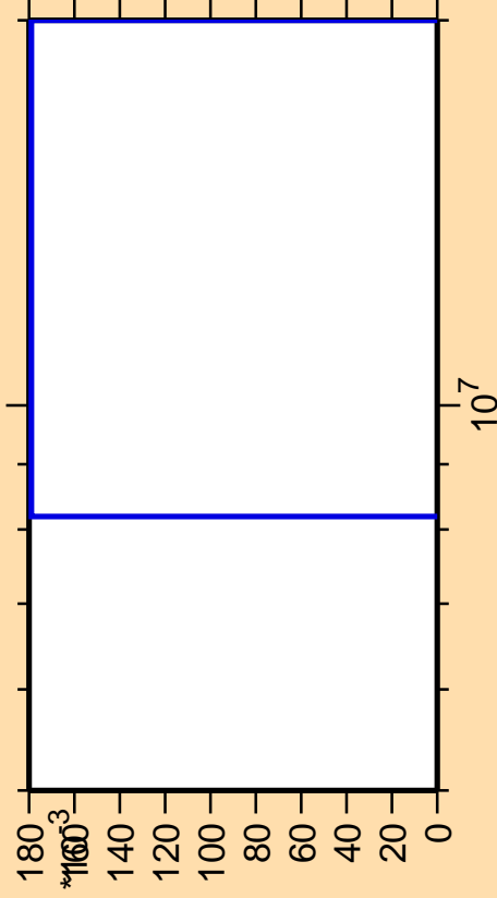
\Delta\sigma/\sigma vs. E for ^{258}\text{Lw}(\text{mt } 42)
