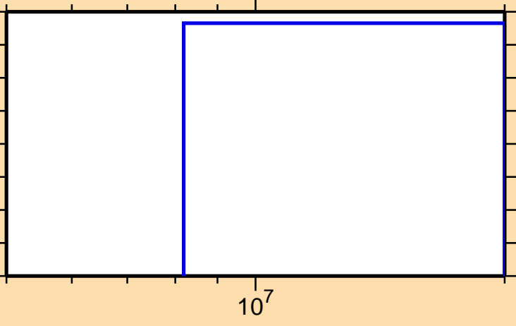
\sigma vs. E for ^{258}\text{Lw}(n,nt)
