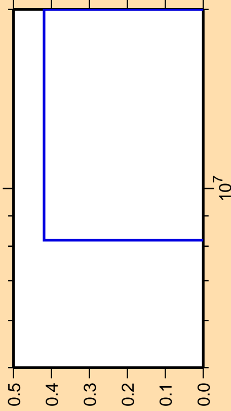
\Delta\sigma/\sigma vs. E for ^{258}\text{Lw}(\text{mt } 34)
