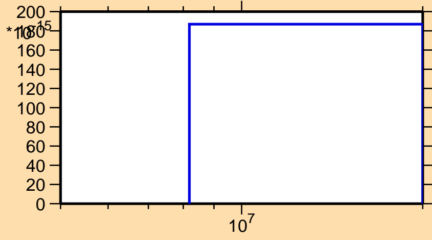
\sigma vs. E for ^{258}\text{Lw}(\text{mt } 42)
