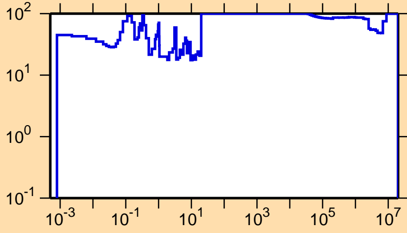
\Delta\sigma/\sigma vs. E for ^{260}\text{Lw}(n,\gamma)
