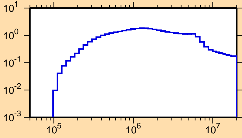
\sigma vs. E for ^{260}\text{Lw}(n,\text{inel.})
