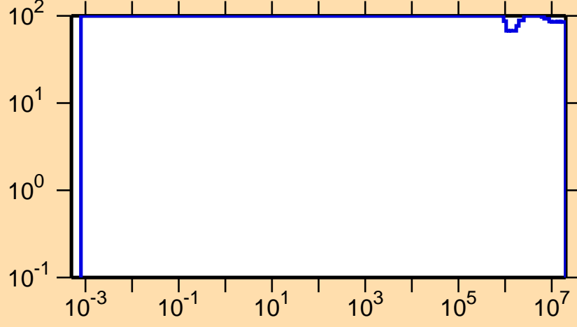
\Delta\sigma/\sigma vs. E for ^{260}\text{Lw}(n,p)
