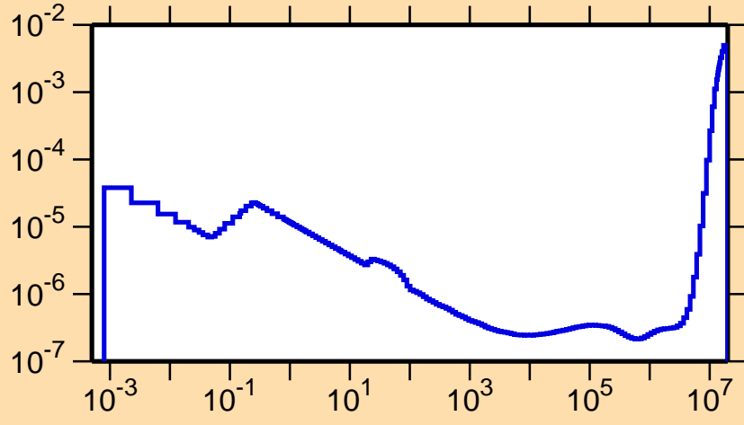
\sigma vs. E for ^{260}\text{Lw}(n,\alpha)
