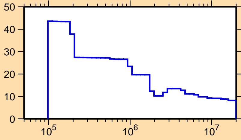
\Delta\sigma/\sigma vs. E for ^{260}\text{Lw}(n,\text{nonel.})
