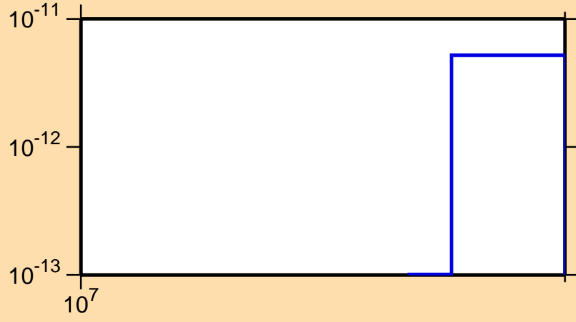
\sigma vs. E for ^{260}\text{Lw}(\text{mt } 34)
