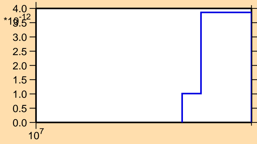
\sigma vs. E for ^{260}\text{Lw} (mt 45)
