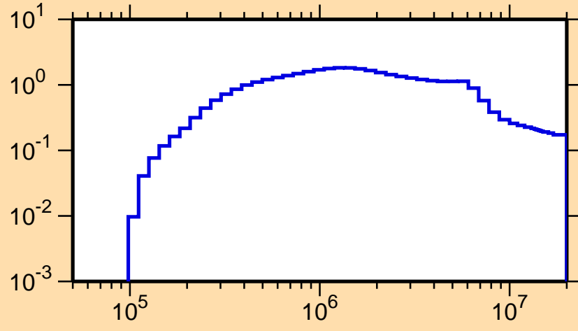
\sigma vs. E for ^{260}\text{Lw}(n,n\text{cont.})
