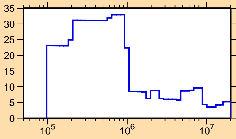
\Delta\sigma/\sigma vs. E for ^{260}\text{Lw}(n,\text{el.})
