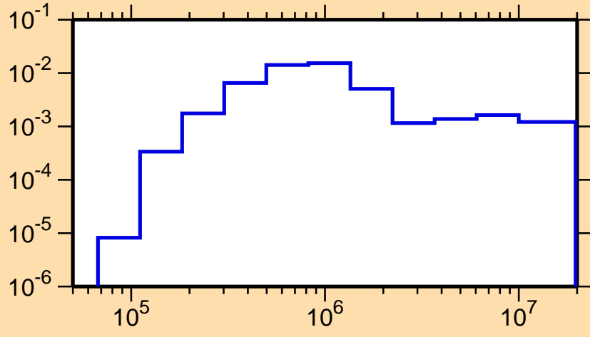
\sigma vs. E for ^{260}\text{Lw}(n,n_1)
