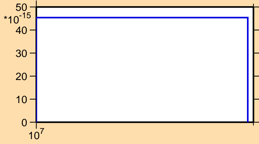
\sigma vs. E for ^{260}\text{Lw}(\text{mt } 42)
