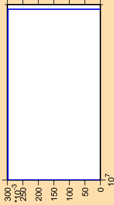
\Delta\sigma/\sigma vs. E for ^{260}\text{Lw}(\text{mt } 11)
