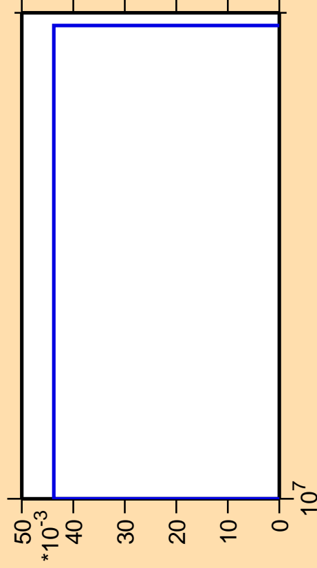
\Delta\sigma/\sigma vs. E for ^{260}\text{Lw}(\text{mt } 42)
