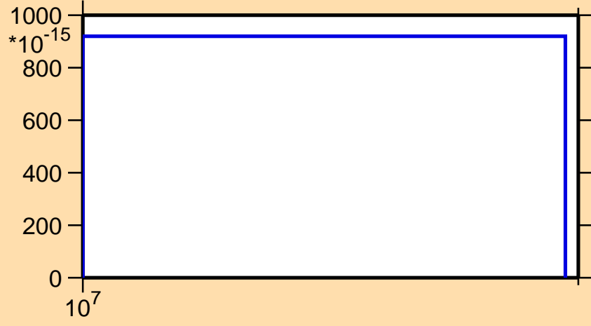
\sigma vs. E for ^{260}\text{Lw}(\text{mt117})
