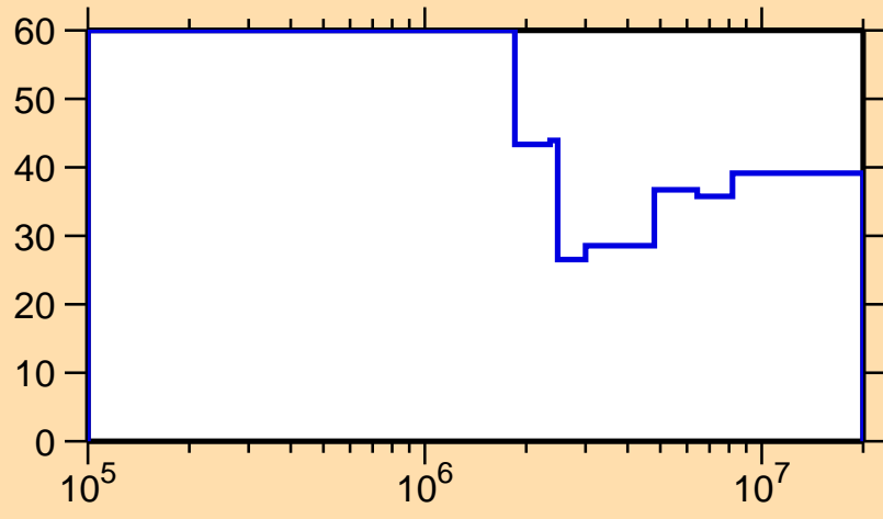
\Delta\sigma/\sigma vs. E for ^{260}\text{Lw}(n, n_1)
