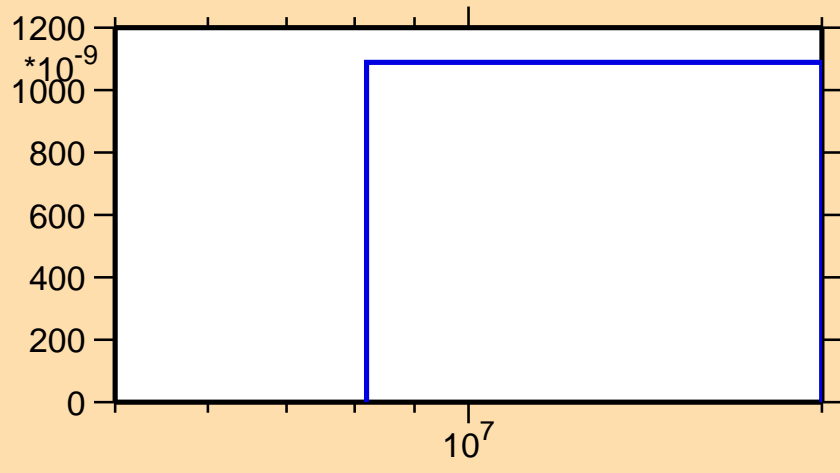
\sigma vs. E for ^{260}\text{Lw}(n,nd)
