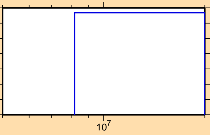
\sigma vs. E for ^{260}\text{Lw}(n,3n)
