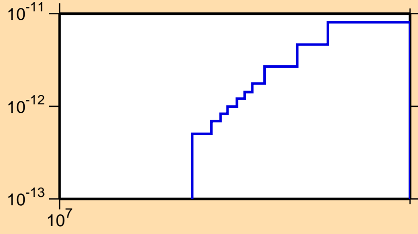
\sigma vs. E for ^{261}\text{Lw}(n,p\alpha)
