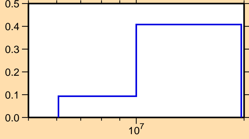
\sigma vs. E for ^{261}\text{Lw}(n,2n)
