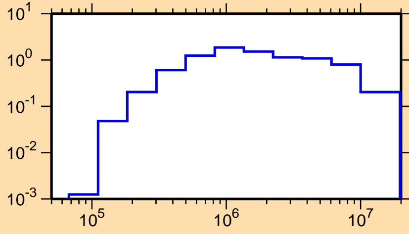
\sigma vs. E for ^{261}\text{Lw}(n,n\text{cont.})
