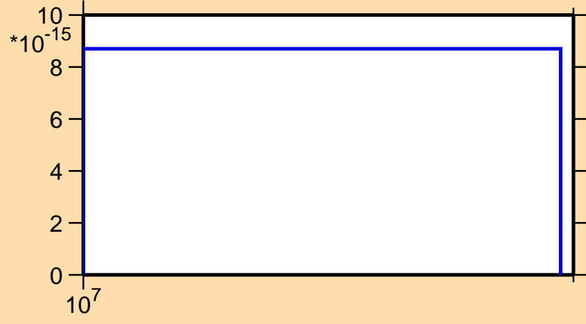
\sigma vs. E for ^{261}\text{Lw}(\text{mt } 42)
