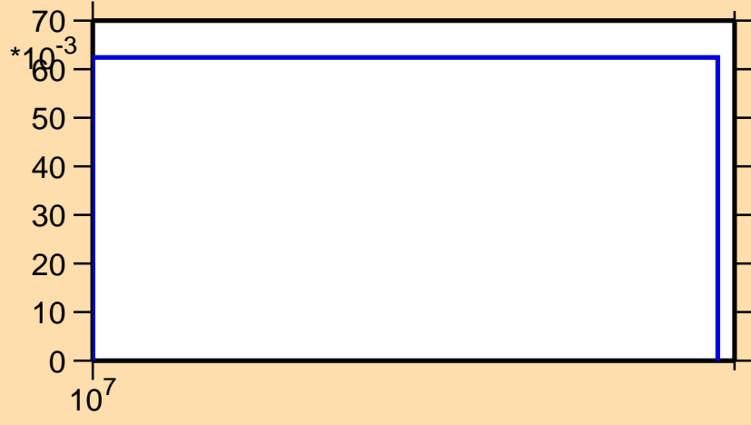
\sigma vs. E for ^{261}\text{Lw}(n,3n)
