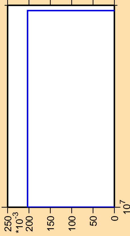
\Delta\sigma/\sigma vs. E for ^{261}\text{Lw}(\text{mt } 45)
