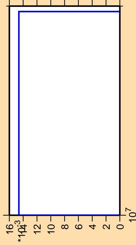
\Delta\sigma/\sigma vs. E for ^{261}\text{Lw}(\text{mt } 42)
