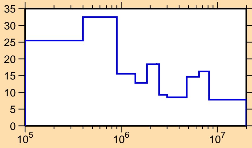
\Delta\sigma/\sigma vs. E for ^{261}\text{Lw}(n,\text{el.})
