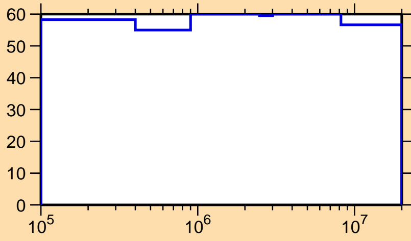
\Delta\sigma/\sigma vs. E for ^{261}\text{Lw}(n,n\text{cont.})
