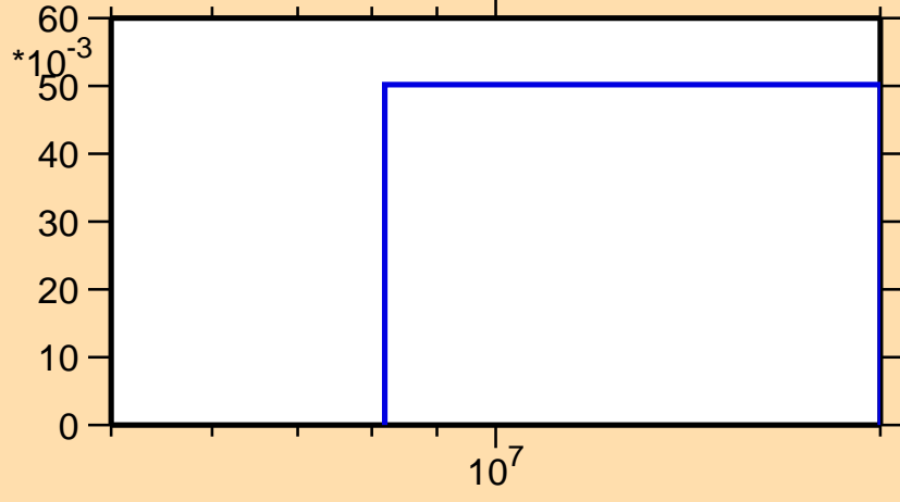
\sigma vs. E for ^{261}\text{Lw}(n,3n)
