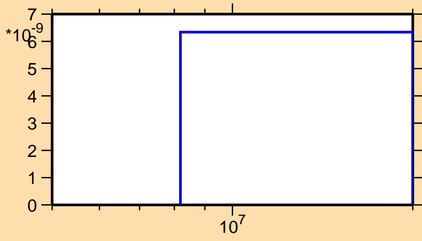
\sigma vs. E for ^{261}\text{Lw}(n,2np)
