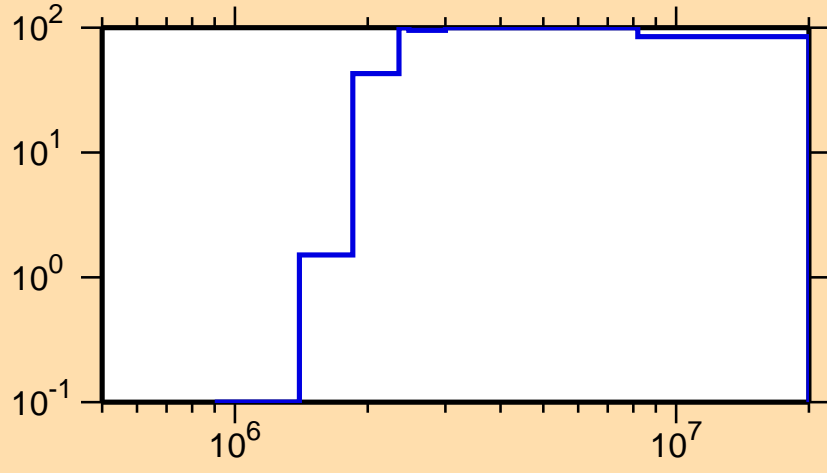
\Delta\sigma/\sigma vs. E for ^{261}\text{Lw}(n,p)
