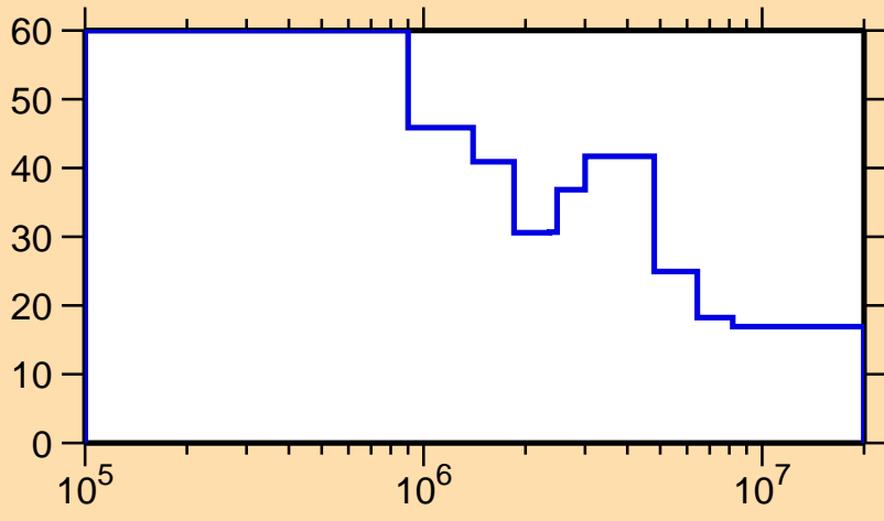
\Delta\sigma/\sigma vs. E for ^{261}\text{Lw}(n,f)
