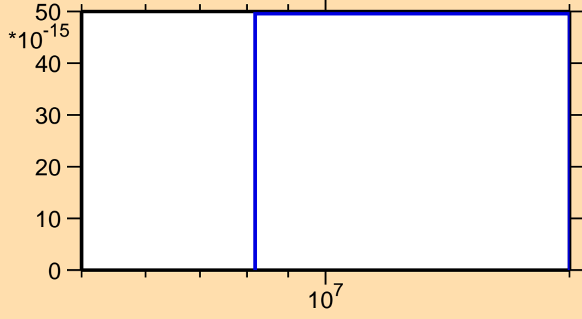
\sigma vs. E for ^{261}\text{Lw}(\text{mt } 11)
