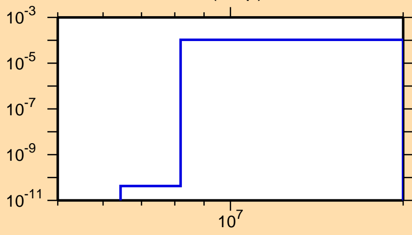
\sigma vs. E for ^{261}\text{Lw}(n,np)
