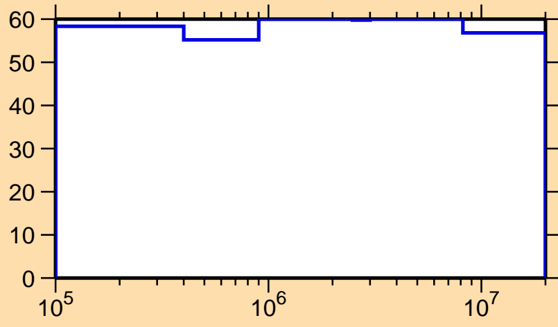
\Delta\sigma/\sigma vs. E for ^{261}\text{Lw}(n,\text{inel.})
