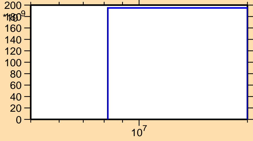
\sigma vs. E for ^{261}\text{Lw}(n,nt)
