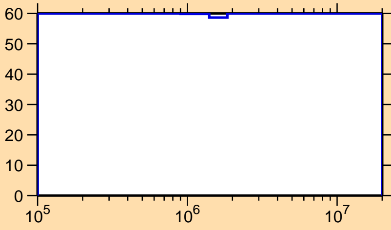
\Delta\sigma/\sigma vs. E for ^{261}\text{Lw}(n,n_1)
