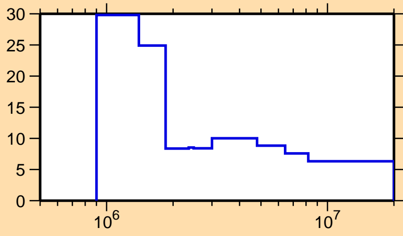
\Delta\sigma/\sigma vs. E for ^{261}\text{Lw}(n,\text{nonel.})
