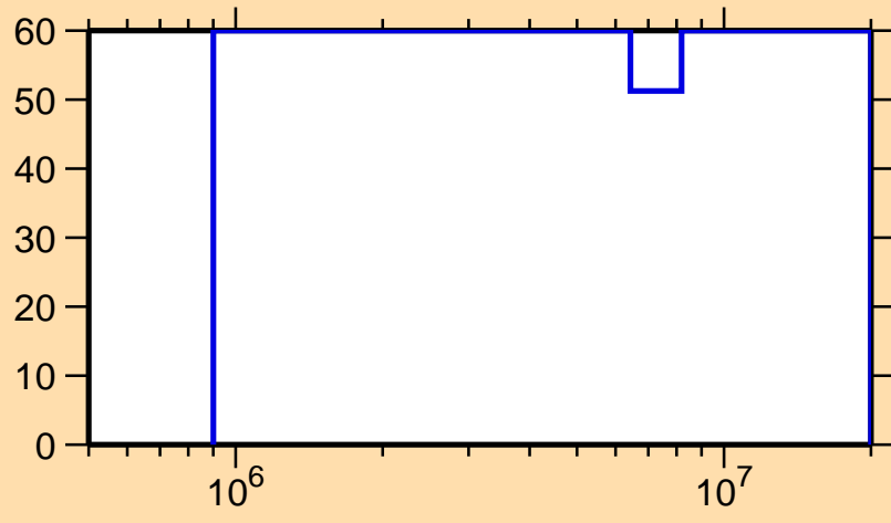
\Delta\sigma/\sigma vs. E for ^{261}\text{Lw}(n,\gamma)
