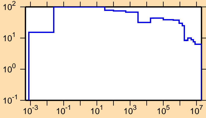
\Delta\sigma/\sigma vs. E for ^{261}\text{Lw}(n,\text{nonel.})
