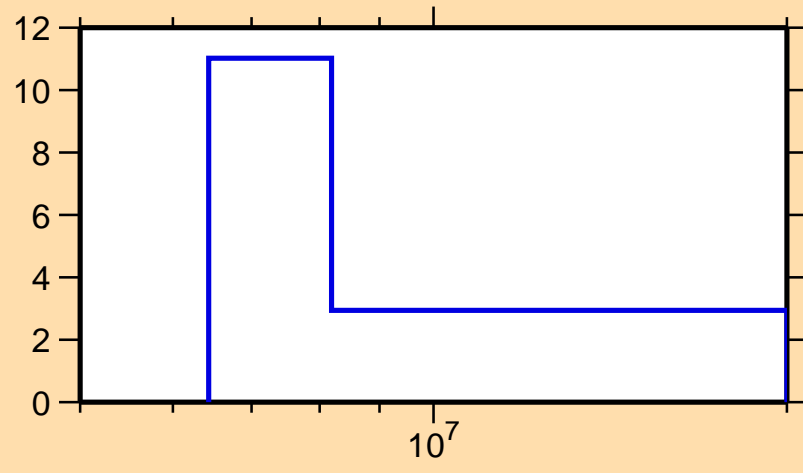
\Delta\sigma/\sigma vs. E for ^{261}\text{Lw}(n,\text{tot.})
