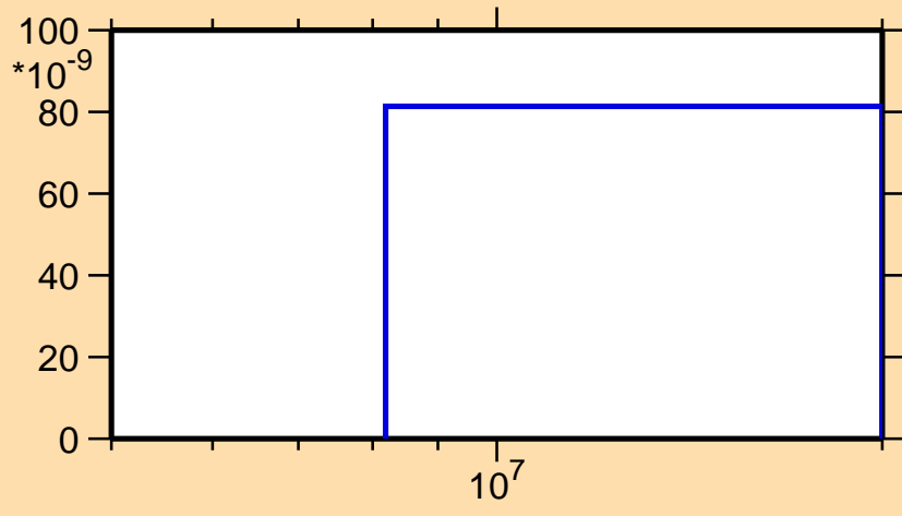
\sigma vs. E for ^{261}\text{Lw}(n,3n\alpha)
