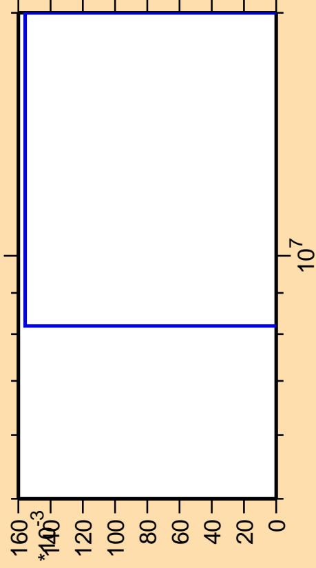
\Delta\sigma/\sigma vs. E for ^{261}\text{Lw}(\text{mt } 11)
