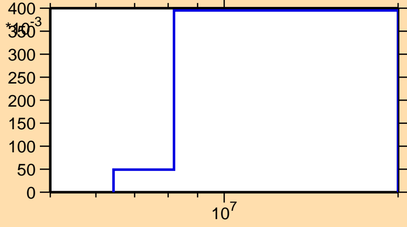
\sigma vs. E for ^{261}\text{Lw}(n,2n)
