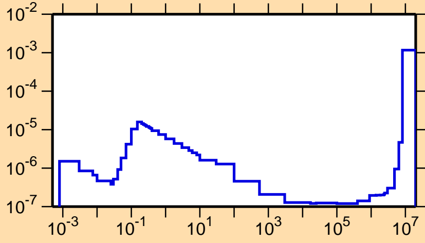
\sigma vs. E for ^{261}\text{Lw}(n,\alpha)
