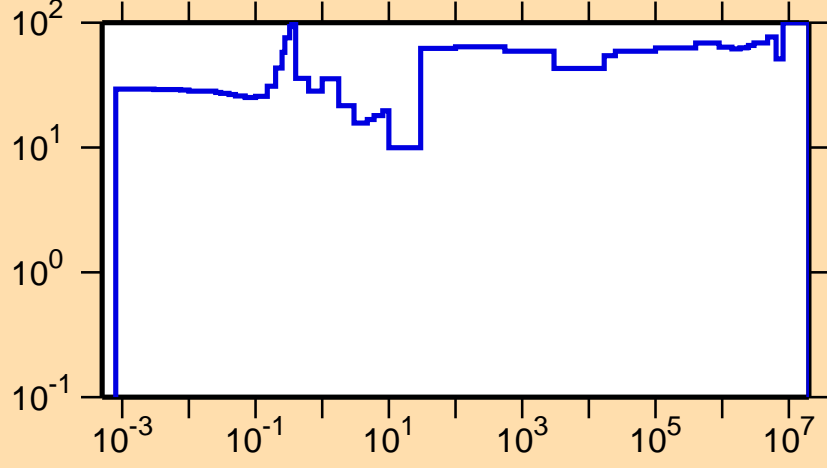
\Delta\sigma/\sigma vs. E for ^{261}\text{Lw}(n,\gamma)
