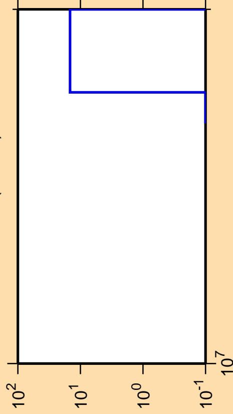
\Delta\sigma/\sigma vs. E for ^{262}\text{Lw}(\text{mt 11})
