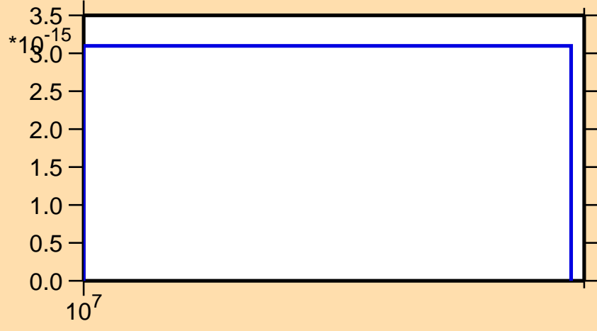
\sigma vs. E for ^{262}\text{Lw} (mt 34)
