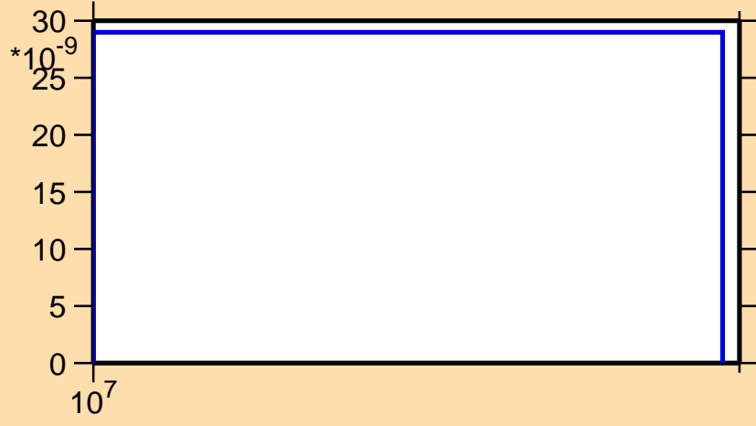
\sigma vs. E for ^{262}\text{Lw}(n,2np)
