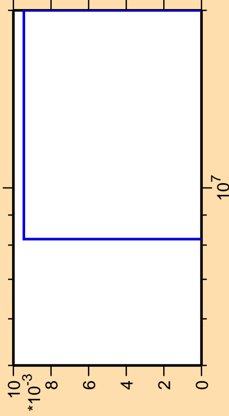
\Delta\sigma/\sigma vs. E for ^{262}\text{Lw}(\text{mt } 42)
