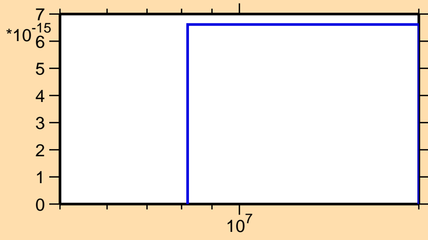
\sigma vs. E for ^{262}\text{Lw}(\text{mt } 42)
