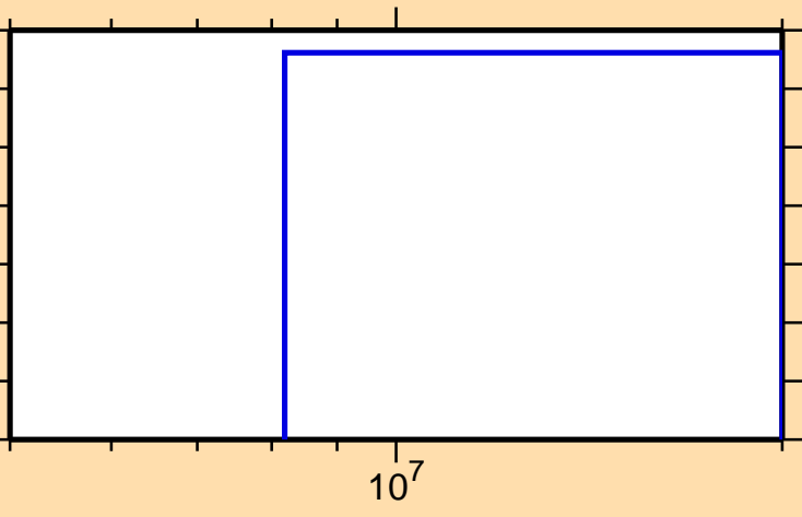
\sigma vs. E for ^{262}\text{Lw}(\text{mt } 42)
