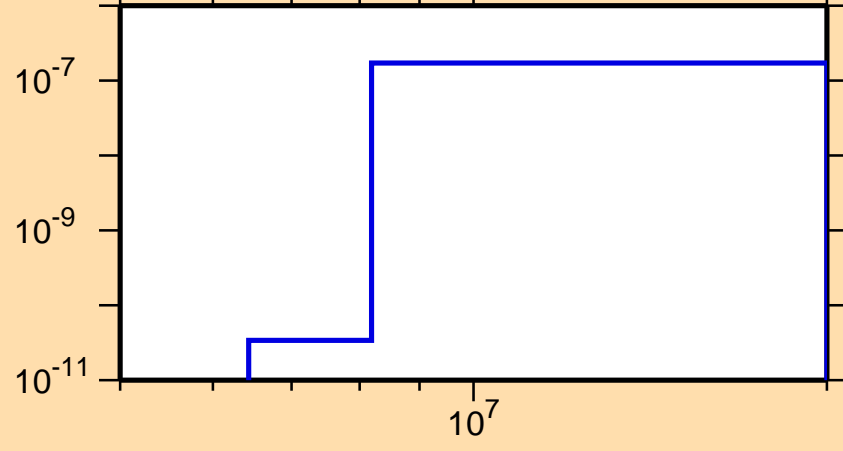
\sigma vs. E for ^{262}\text{Lw}(n,2n\alpha)
