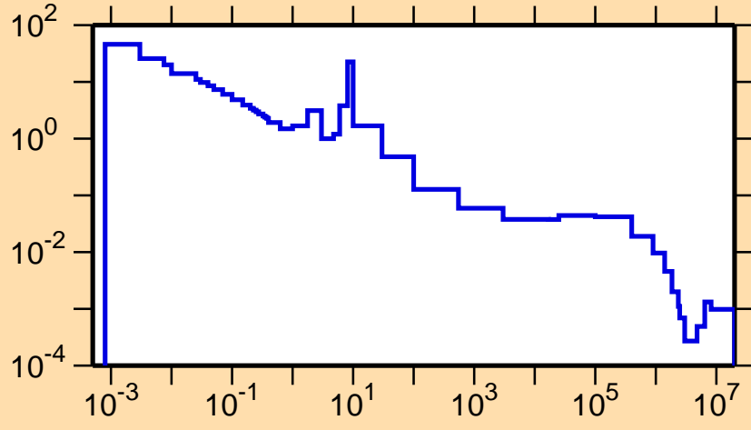
\sigma vs. E for ^{262}\text{Lw}(n,\gamma)
