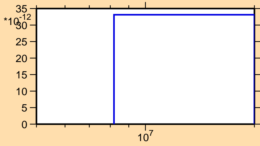
\sigma vs. E for ^{262}\text{Lw}(n,\text{He3})
