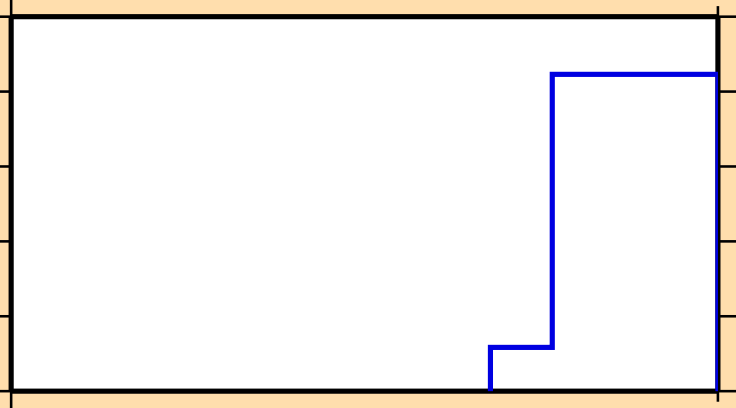
\sigma vs. E for ^{263}\text{Lw} (mt 11)
