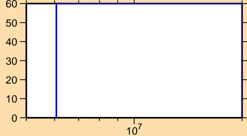
\Delta\sigma/\sigma vs. E for ^{263}\text{Lw}(n, 2n)
