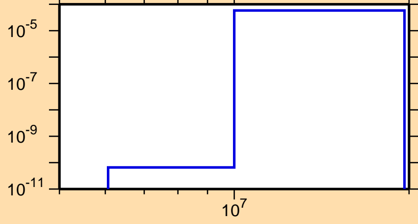
\sigma vs. E for ^{263}\text{Lw}(n,t)
