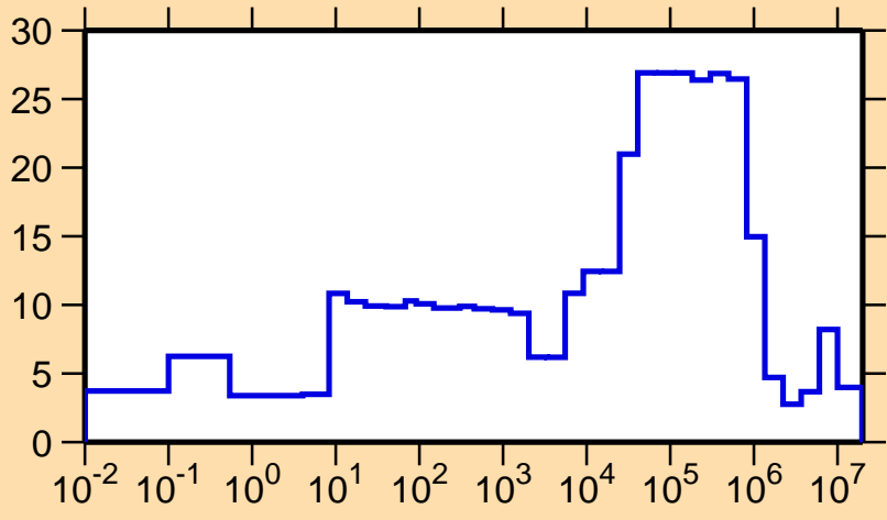
\Delta\sigma/\sigma vs. E for ^{263}\text{Lw}(n,\text{tot.})
