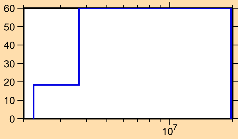
\Delta\sigma/\sigma vs. E for ^{263}\text{Lw}(n,p)
