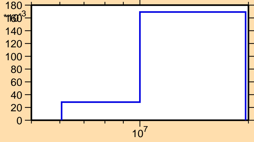
\sigma vs. E for ^{263}\text{Lw}(n,2n)
