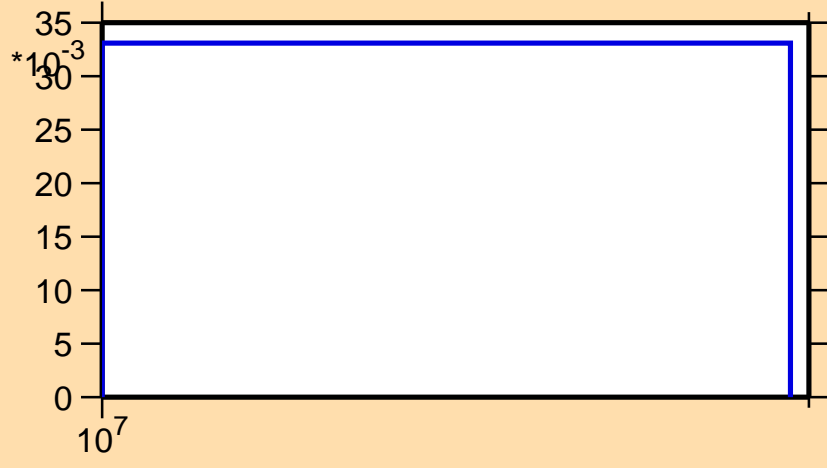
\sigma vs. E for ^{263}\text{Lw}(n,3n)
