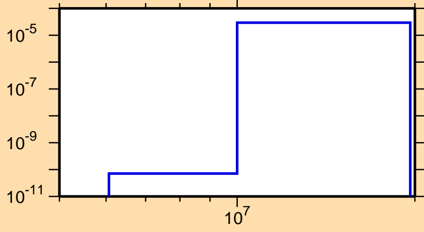
\sigma vs. E for ^{263}\text{Lw}(n,np)
