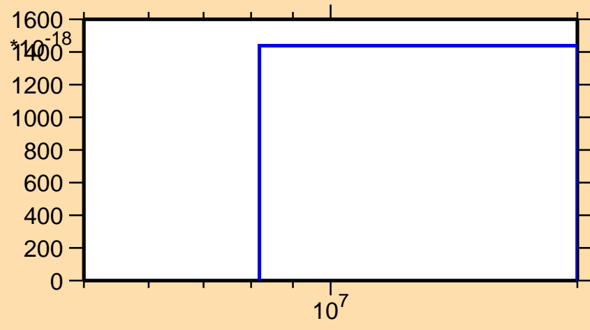
\sigma vs. E for ^{263}\text{Lw}(\text{mt } 42)
