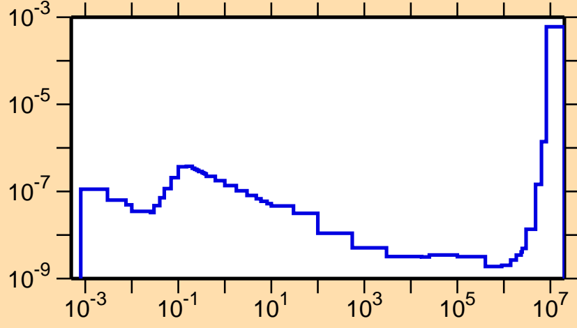
\sigma vs. E for ^{263}\text{Lw}(n,\alpha)
