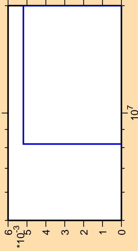
\Delta\sigma/\sigma vs. E for ^{263}\text{Lw}(\text{mt } 42)
