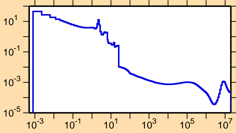
\sigma vs. E for ^{264}\text{Lw}(n,\gamma)
