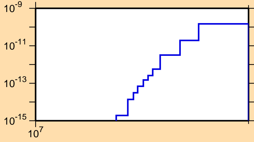
\sigma vs. E for ^{264}\text{Lw}(n,3n\alpha)
