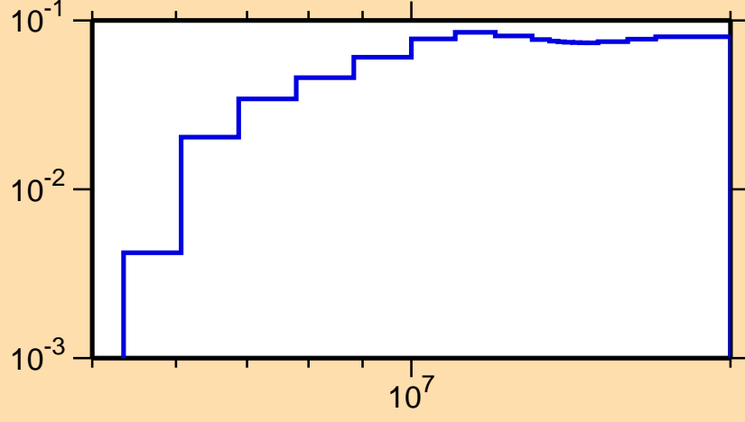
\sigma vs. E for ^{264}\text{Lw}(n,2n)
