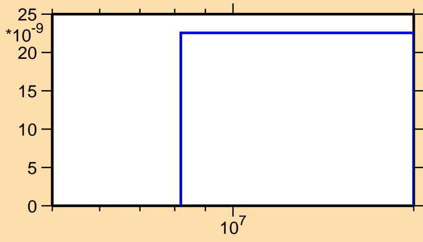
\sigma vs. E for ^{264}\text{Lw}(n,nd)
