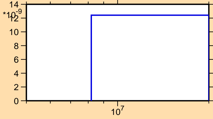
\sigma vs. E for ^{264}\text{Lw}(n,2n\alpha)
