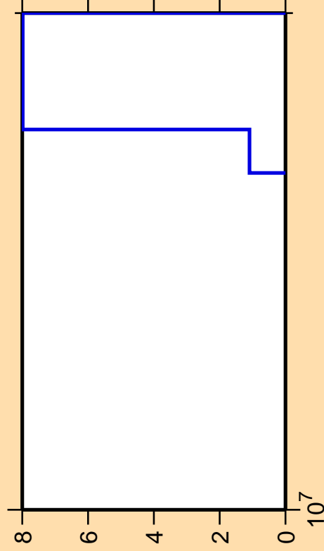
\Delta\sigma/\sigma vs. E for ^{265}\text{Lw}(n,3n\alpha)
