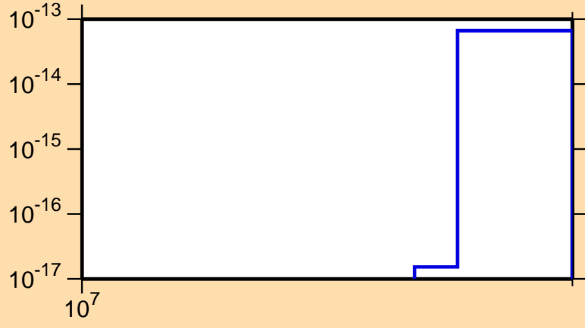
\sigma vs. E for ^{265}\text{Lw}(\text{mt } 11)
