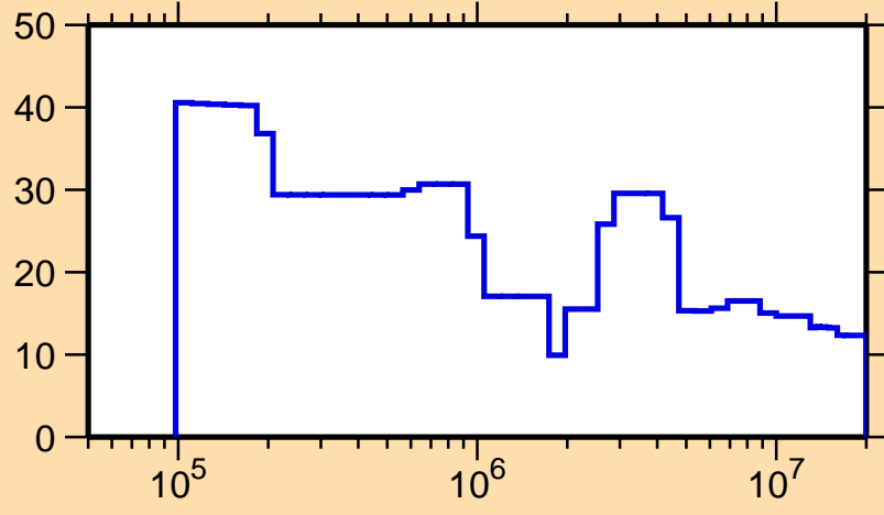
\Delta\sigma/\sigma vs. E for ^{265}\text{Lw}(n,f)
