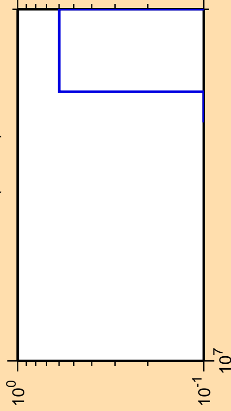
\Delta\sigma/\sigma vs. E for ^{265}\text{Lw}(\text{mt } 11)
