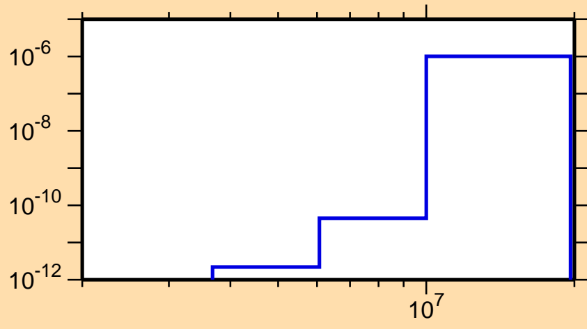
\sigma vs. E for ^{265}\text{Lw}(n,n\alpha)
