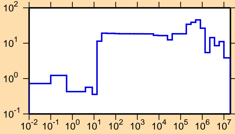
\Delta\sigma/\sigma vs. E for ^{265}\text{Lw}(n,el.)
