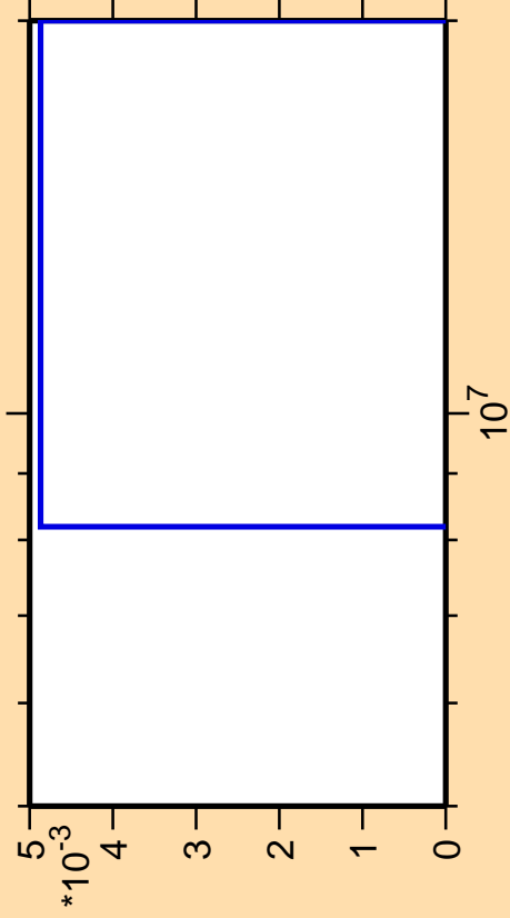
\Delta\sigma/\sigma vs. E for ^{265}\text{Lw}(\text{mt } 11)
