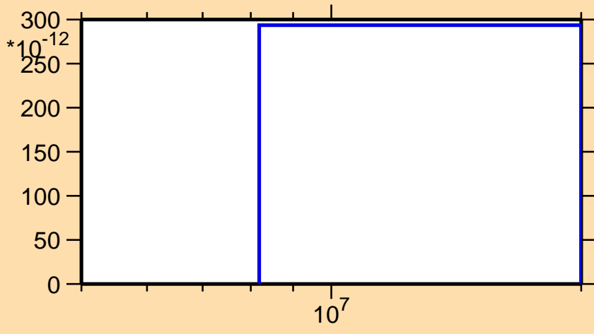
\sigma vs. E for ^{265}\text{Lw}(n,2n\alpha)
