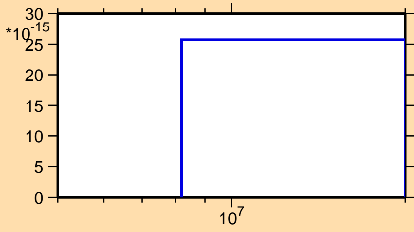
\sigma vs. E for ^{265}\text{Lw}(n,\text{He3})
