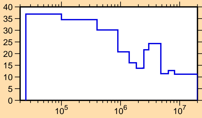
\Delta\sigma/\sigma vs. E for ^{265}\text{Lw}(n,\text{nonel.})
