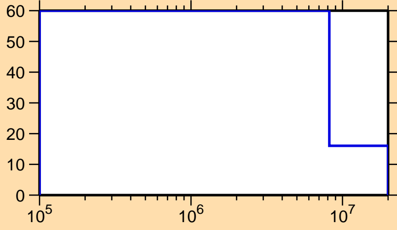
\Delta\sigma/\sigma vs. E for ^{265}\text{Lw}(n,n_1)
