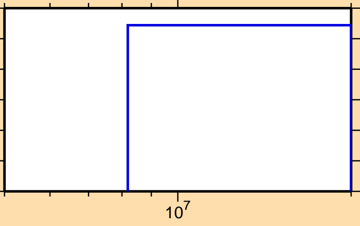
\sigma vs. E for ^{265}\text{Lw}(\text{mt } 11)
