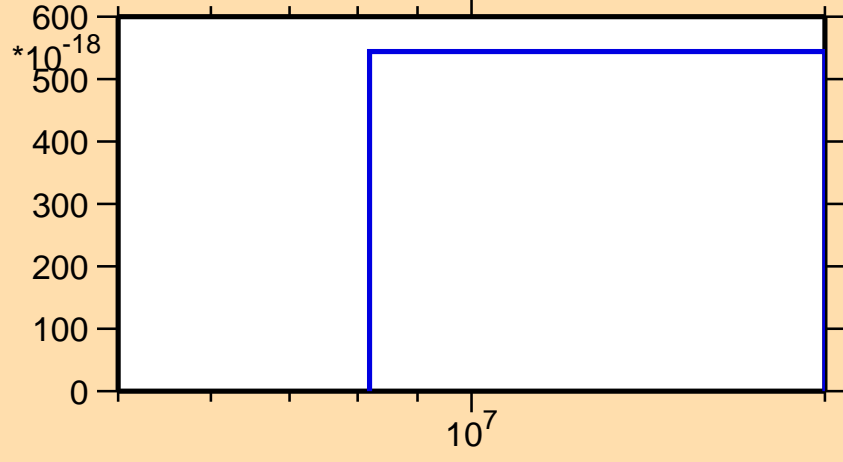
\sigma vs. E for ^{265}\text{Lw}(\text{mt } 11)
