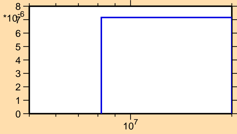
\sigma vs. E for ^{265}\text{Lw}(n,np)
