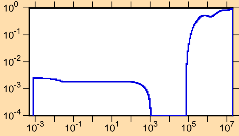
\mu vs. E for ^{266}\text{Lw}(\text{mt251})
