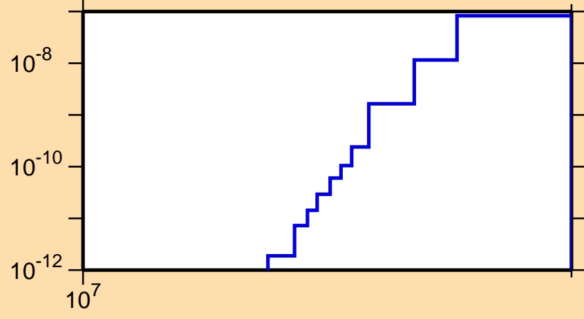
\sigma vs. E for ^{266}\text{Lw}(n,nd)
