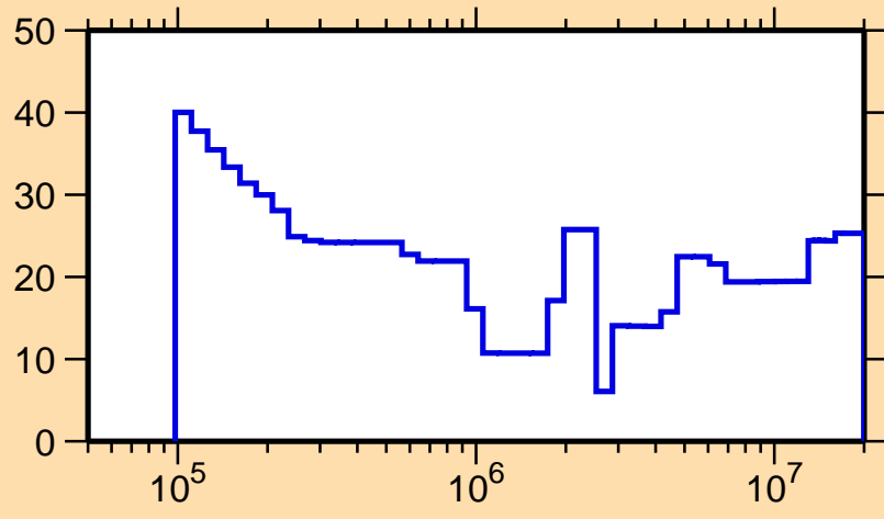
\Delta\sigma/\sigma vs. E for ^{266}\text{Lw}(n,n_1)
