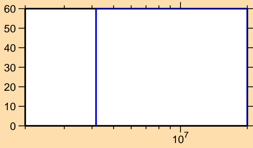
\Delta\sigma/\sigma vs. E for ^{266}\text{Lw}(n,2n)
