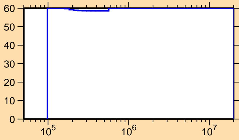
\Delta\sigma/\sigma vs. E for ^{266}\text{Lw}(n, n\text{cont.})
