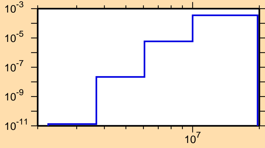
\sigma vs. E for ^{266}\text{Lw}(n,p)
