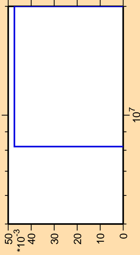
\Delta\sigma/\sigma vs. E for ^{266}\text{Lw}(n,3n\alpha)
