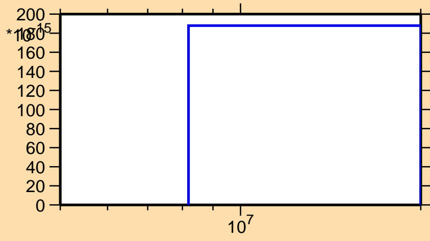
\sigma vs. E for ^{266}\text{Lw}(n,\text{He3})
