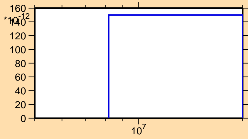
\sigma vs. E for ^{266}\text{Lw}(n,2n\alpha)
