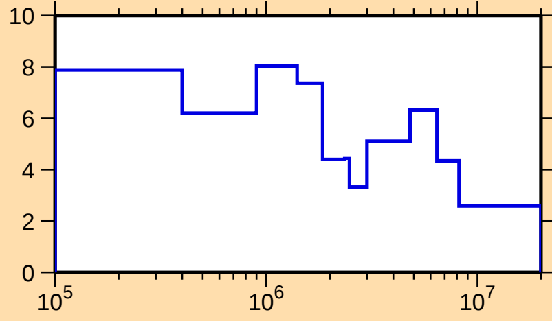
\Delta\sigma/\sigma vs. E for ^{154}\text{Lu}(n,\text{tot.})
