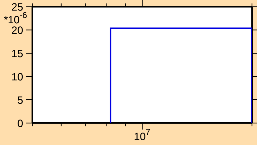
\sigma vs. E for ^{154}\text{Lu}(n,\text{pt})
