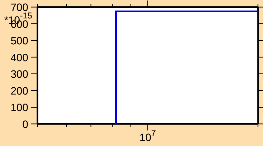
\sigma vs. E for ^{154}\text{Lu}(n,nt)
