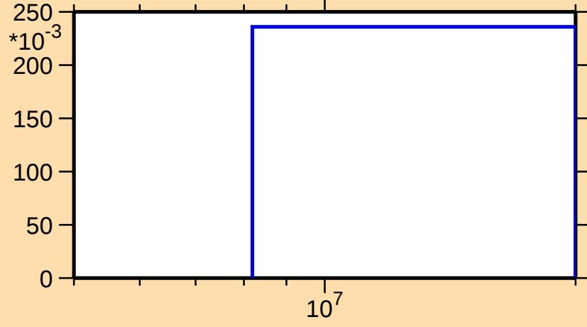
\sigma vs. E for ^{158}\text{Lu}(n,2n)
