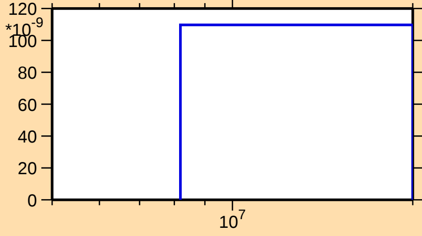
\sigma vs. E for ^{158}\text{Lu}(n,\text{pt})
