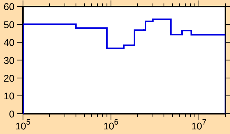
\Delta\sigma/\sigma vs. E for ^{158}\text{Lu}(n,n_1)
