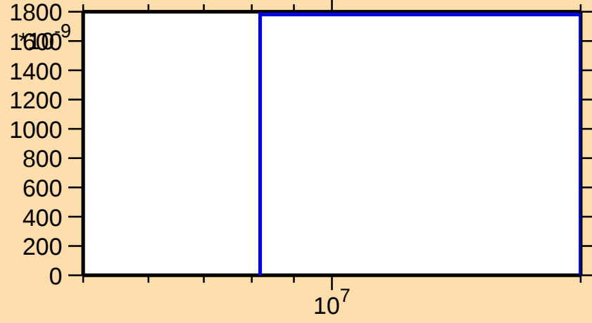
\sigma vs. E for ^{158}\text{Lu}(n,\text{pd})
