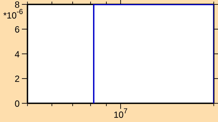
\sigma vs. E for ^{158}\text{Lu}(n,\text{nd})
