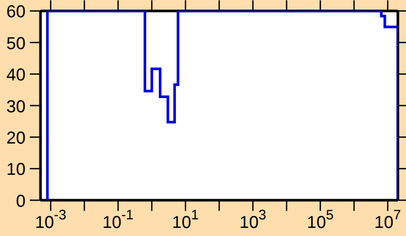
\Delta\sigma/\sigma vs. E for ^{158}\text{Lu}(n,\gamma)
