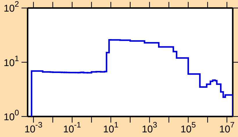
\sigma vs. E for ^{158}\text{Lu}(n,\text{el.})
