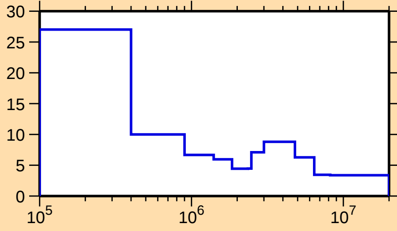
\Delta\sigma/\sigma vs. E for ^{158}\text{Lu}(n,\text{tot.})
