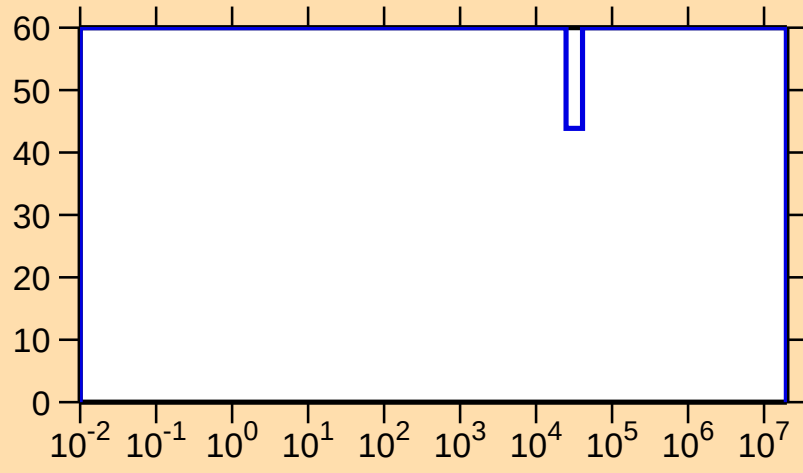
\Delta\sigma/\sigma vs. E for ^{160}\text{Lu}(n,p)
