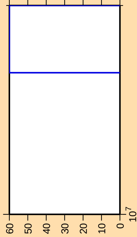
\Delta\sigma/\sigma vs. E for ^{162}\text{Lu}(n,\text{nt})
