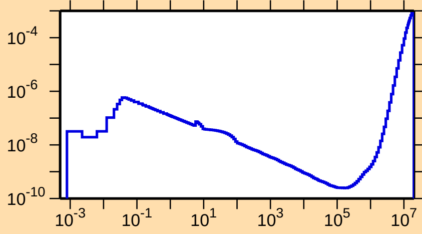
\sigma vs. E for ^{162}\text{Lu}(n,p\alpha)
