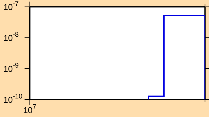
\sigma vs. E for ^{162}\text{Lu}(n,\text{nt})
