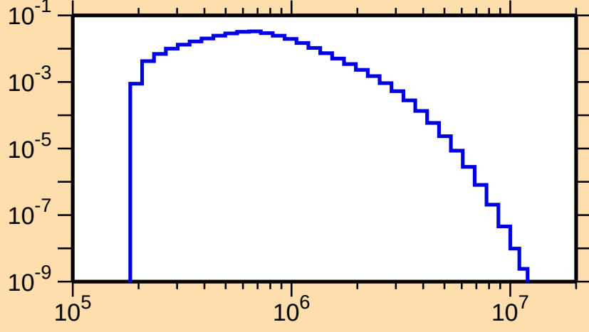
\sigma vs. E for ^{162}\text{Lu}(n,n_4)
