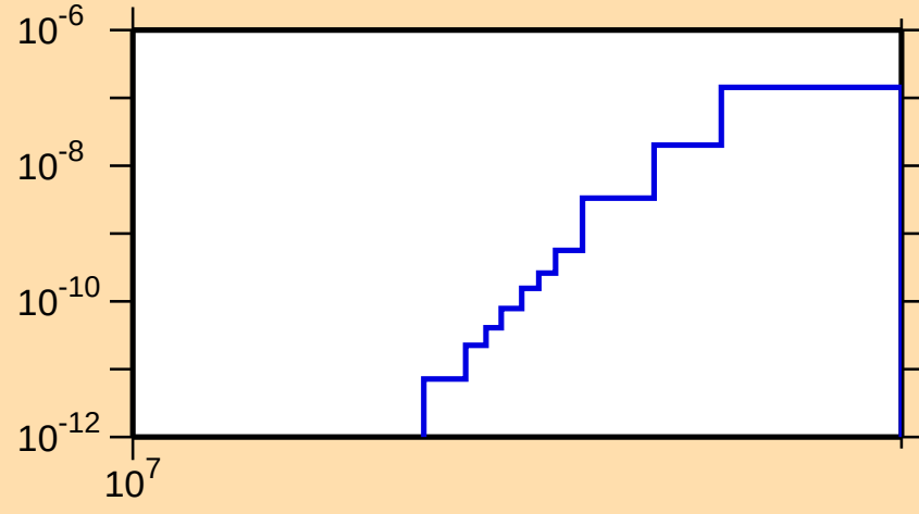
\sigma vs. E for ^{162}\text{Lu}(n,\text{pd})
