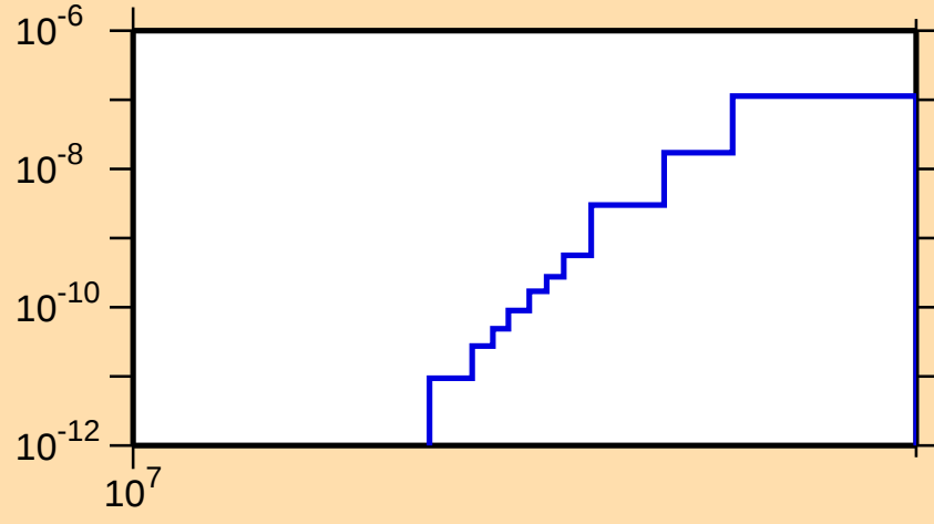
\sigma vs. E for ^{162}\text{Lu}(n,\text{pd})
