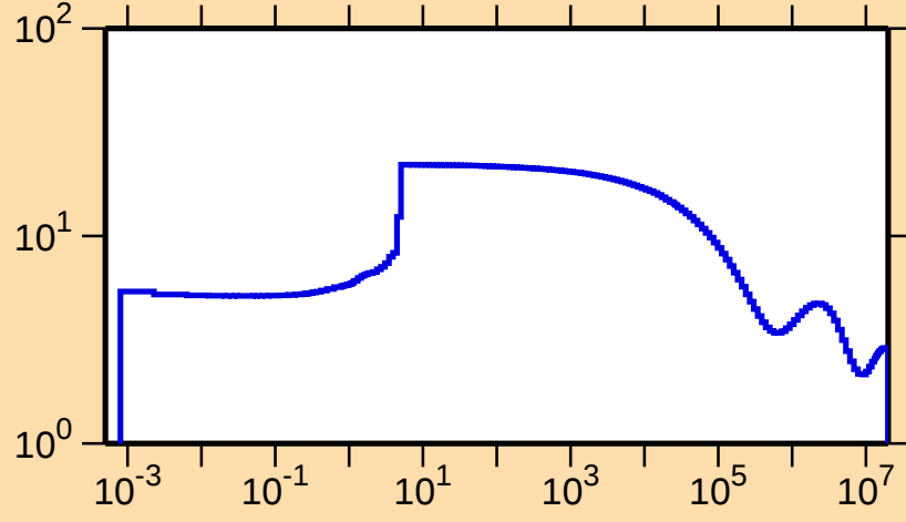
\sigma vs. E for ^{162}\text{Lu}(n,\text{el.})
