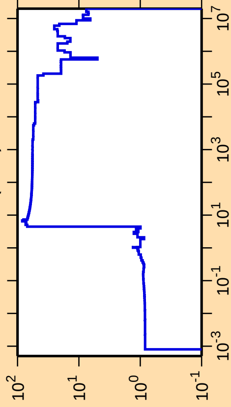
\Delta\sigma/\sigma vs. E for ^{162}\text{Lu}(n,\text{el.})
