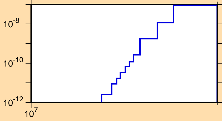
\sigma vs. E for ^{163}\text{Lu}(n,\text{pd})
