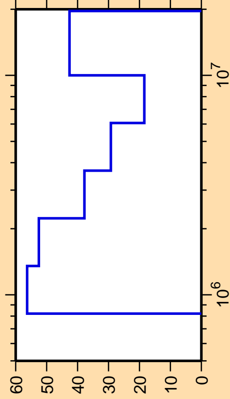
\Delta\sigma/\sigma vs. E for ^{163}\text{Lu}(n,n\text{cont.})
